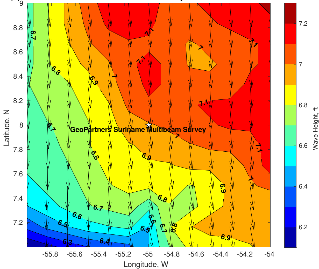
Wave Height (ft) for GeoPartners Suriname Multibeam Survey at 08-Jan-2025 09:00:00
