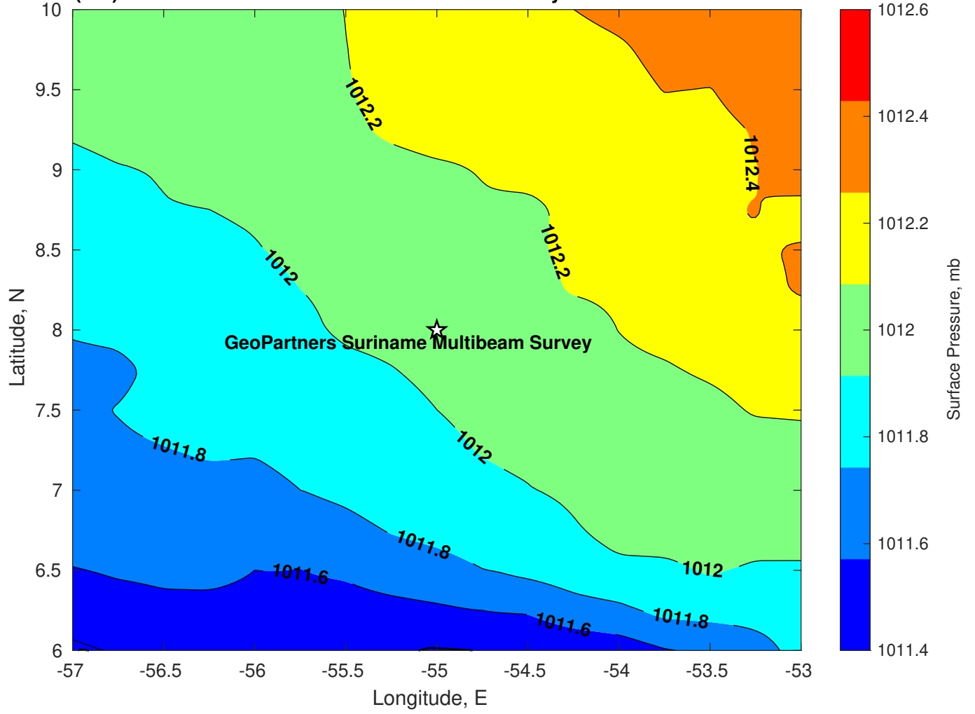
Surface Pressure (mb) for GeoPartners Suriname Multibeam Survey at 10-Jan-2025 00:00:00
