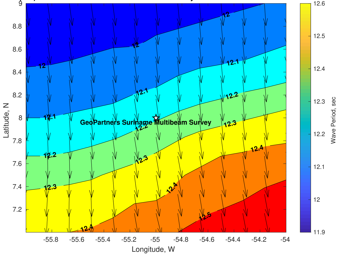
Wave Period (sec) for GeoPartners Suriname Multibeam Survey at 08-Jan-2025 09:00:00
