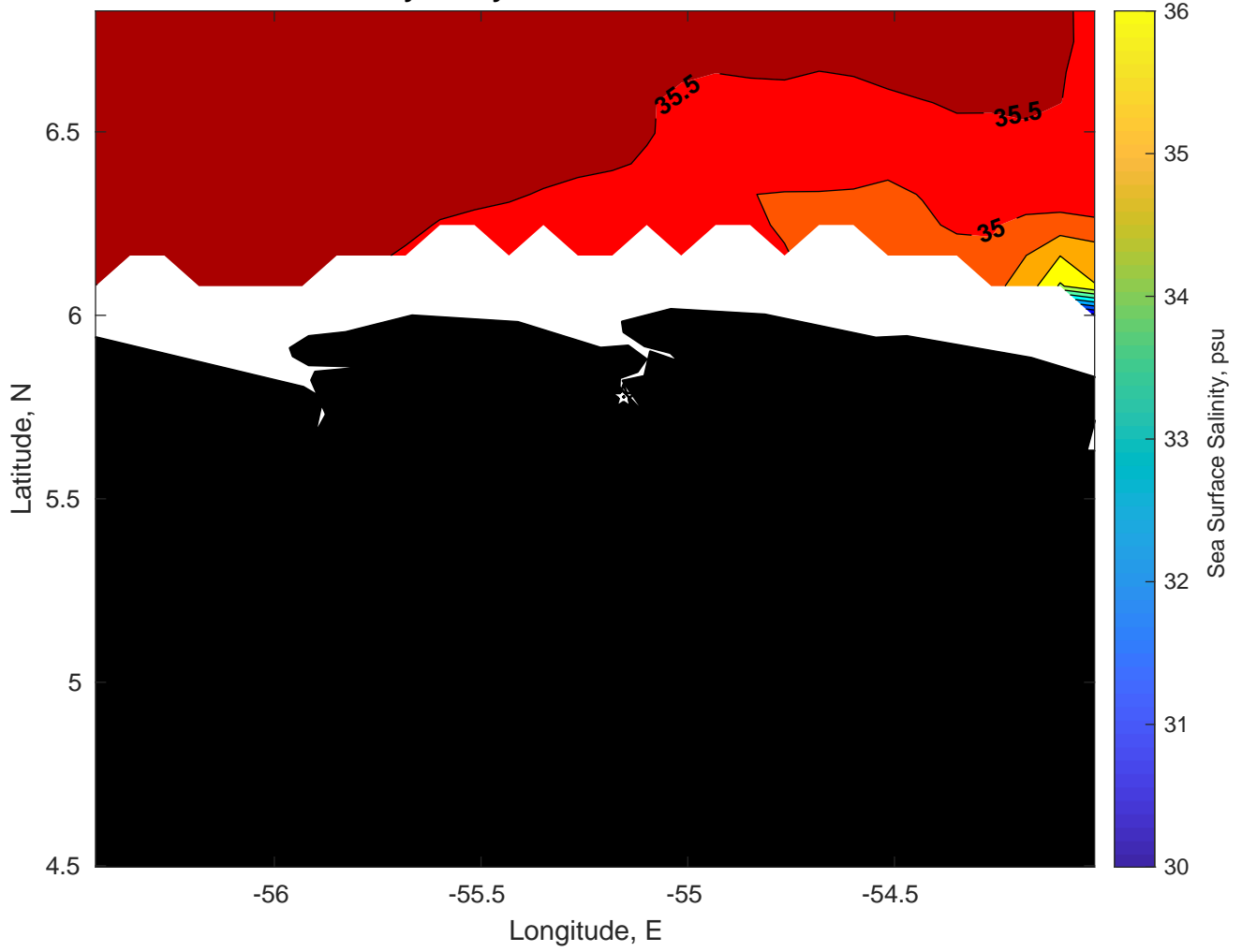
Surface Salinity for Gyre at 07-Jan-2025 00:00:00
