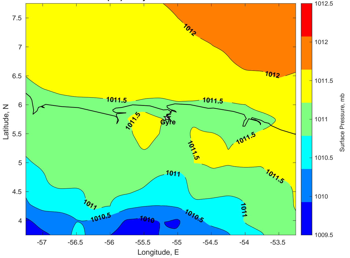
Surface Pressure (mb) for Gyre at 10-Jan-2025 00:00:00
