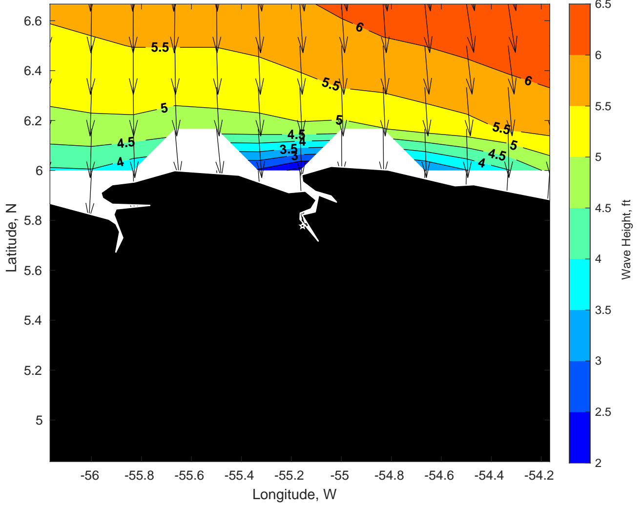
Wave Height (ft) for Gyre at 08-Jan-2025 09:00:00
