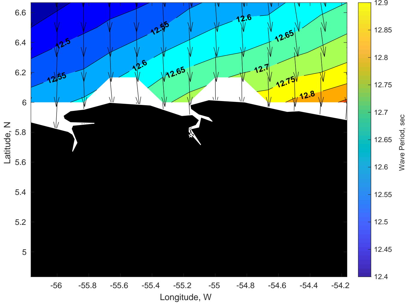
Wave Period (sec) for Gyre at 08-Jan-2025 09:00:00
