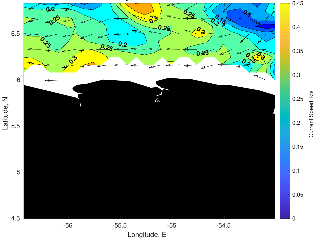
Surface Currents for Gyre at 07-Jan-2025 00:00:00
