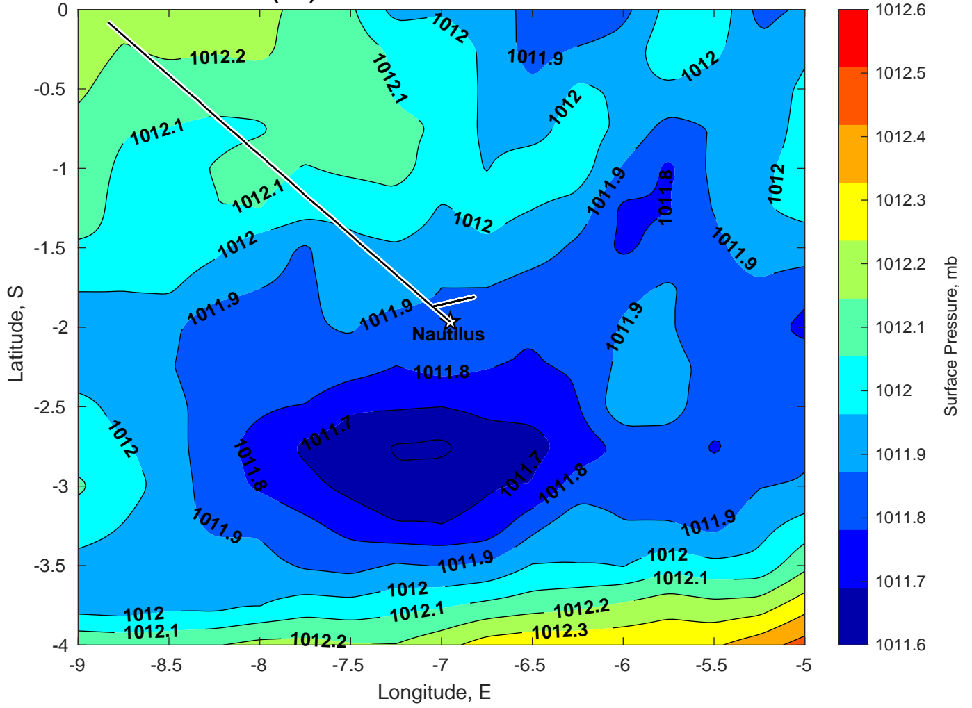
Surface Pressure (mb) for Nautilus at 08-Jan-2025 00:00:00
