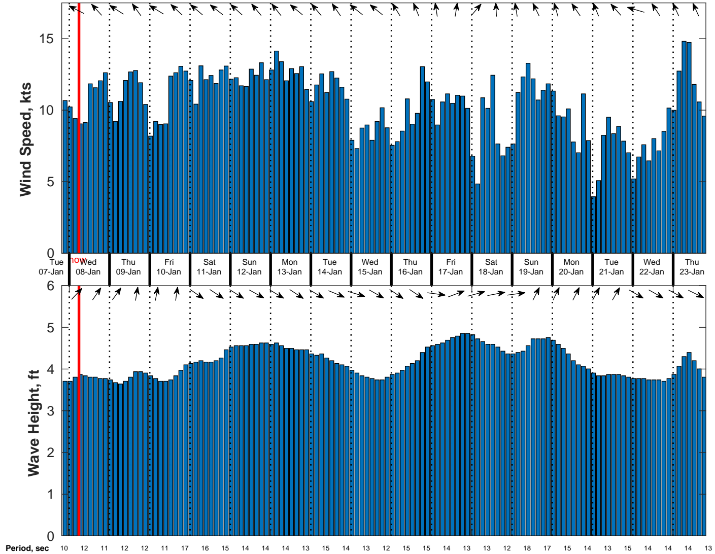
Wind & Wave Forecast for Nautilus from 07-Jan-2025 20:00:00 to 23-Jan-2025 20:00:00
