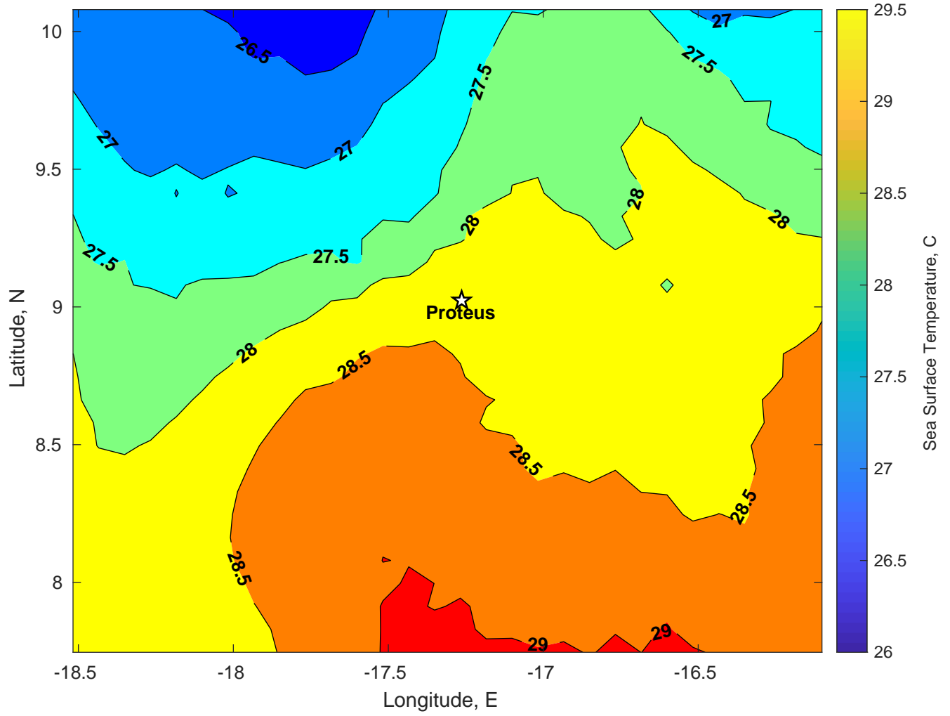
SST for Proteus at 07-Jan-2025 00:00:00
