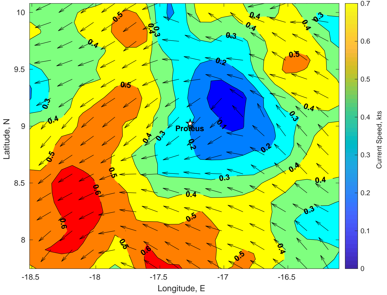
Surface Currents for Proteus at 07-Jan-2025 00:00:00
