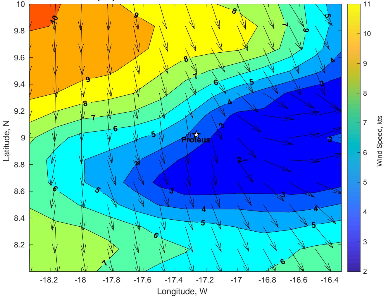
Winds (kts) for Proteus at 08-Jan-2025 09:00:00
