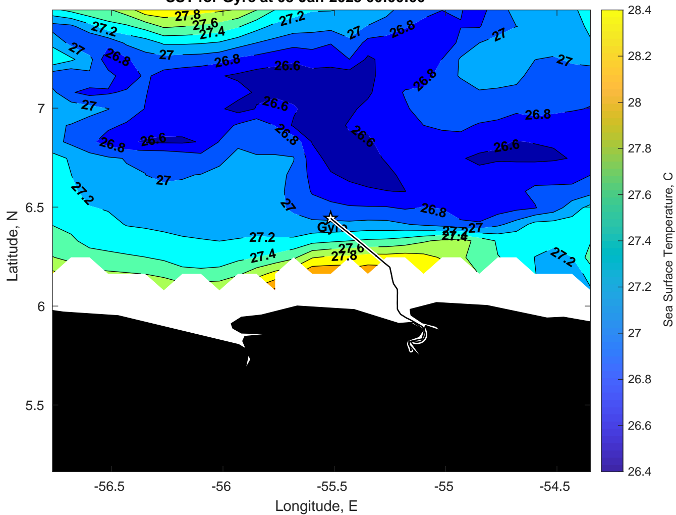
SST for Gyre at 08-Jan-2025 00:00:00
