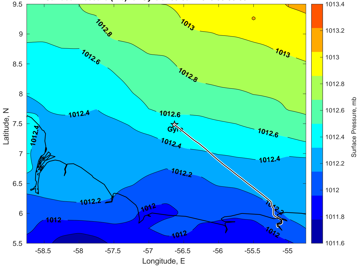
Surface Pressure (mb) for Gyre at 09-Jan-2025 00:00:00
