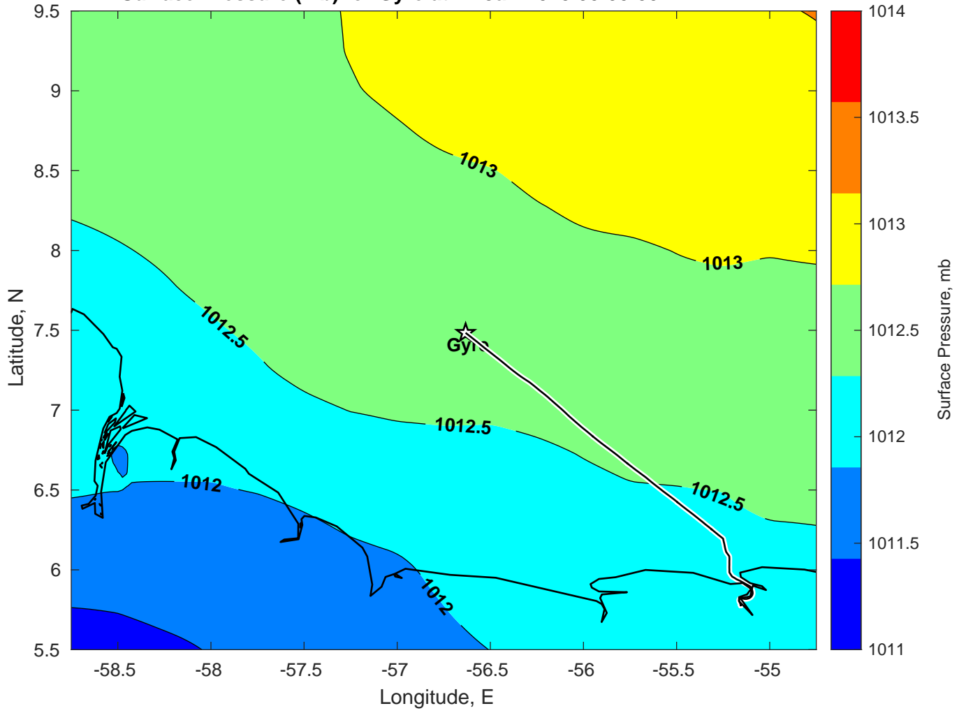
Surface Pressure (mb) for Gyre at 11-Jan-2025 00:00:00
