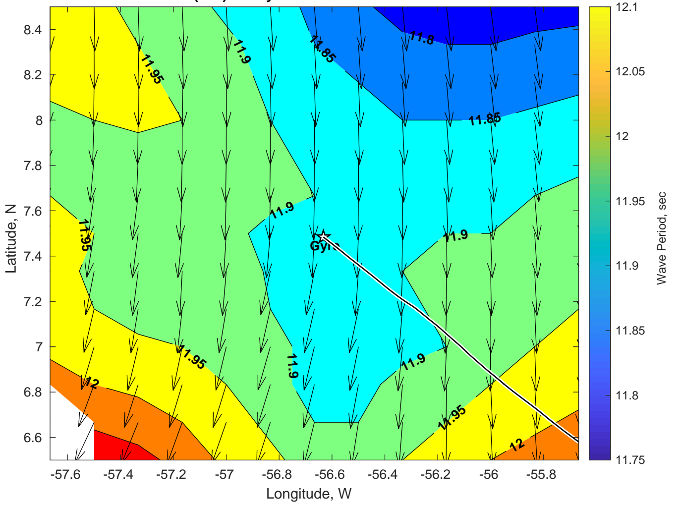
Wave Period (sec) for Gyre at 09-Jan-2025 09:00:00
