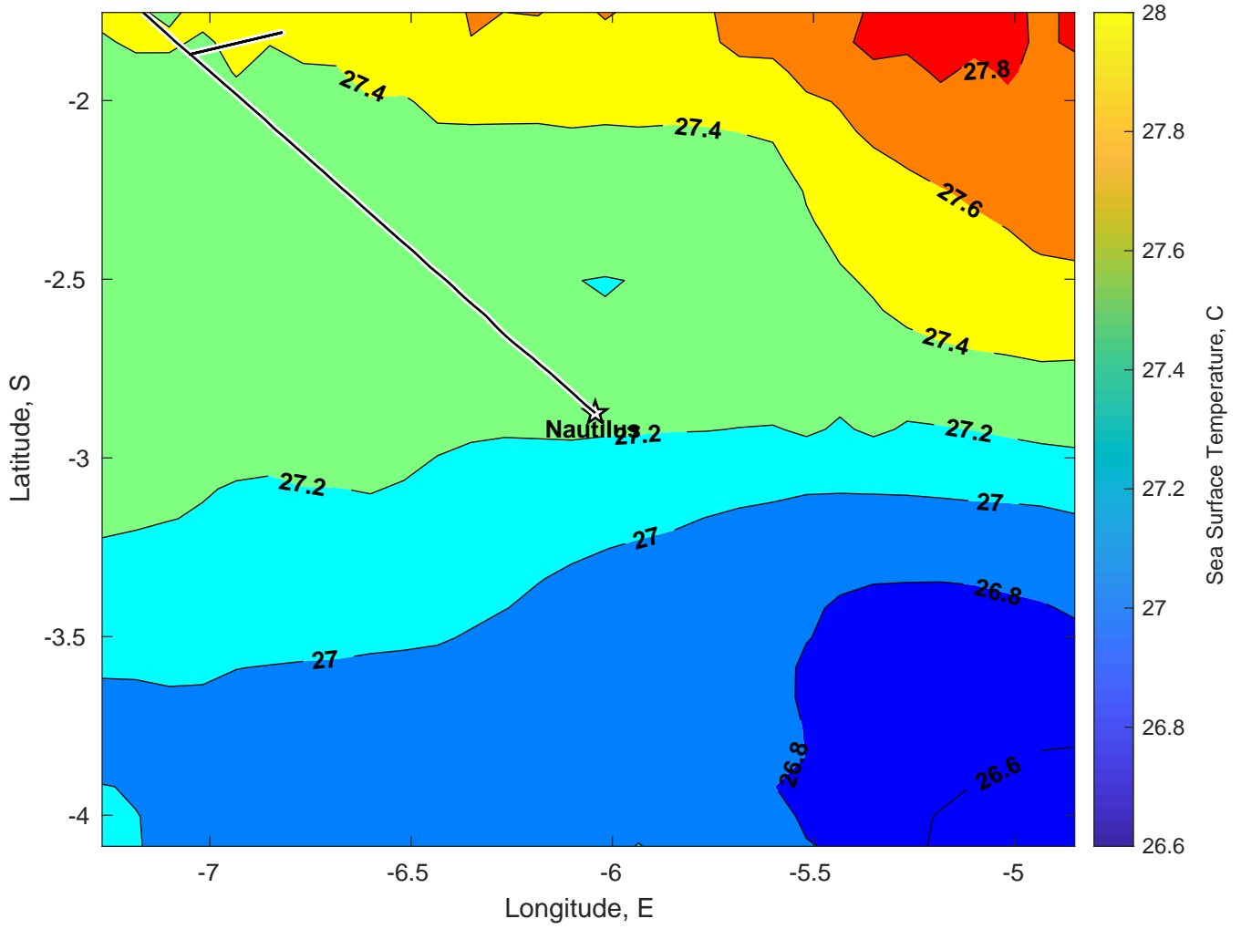
SST for Nautilus at 08-Jan-2025 00:00:00
