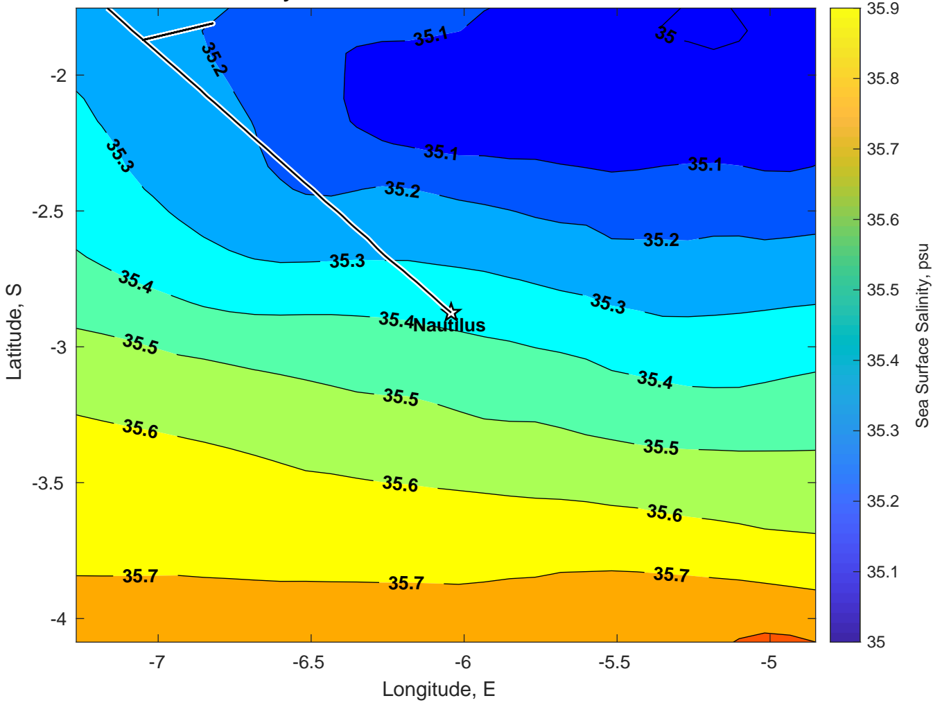
Surface Salinity for Nautilus at 08-Jan-2025 00:00:00
