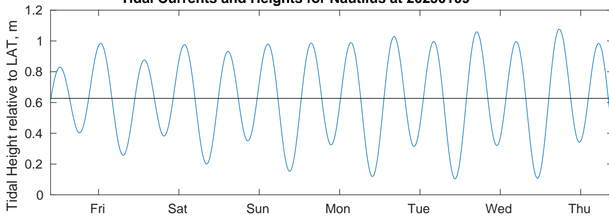
Tidal Currents and Heights for Nautilus at 20250109
