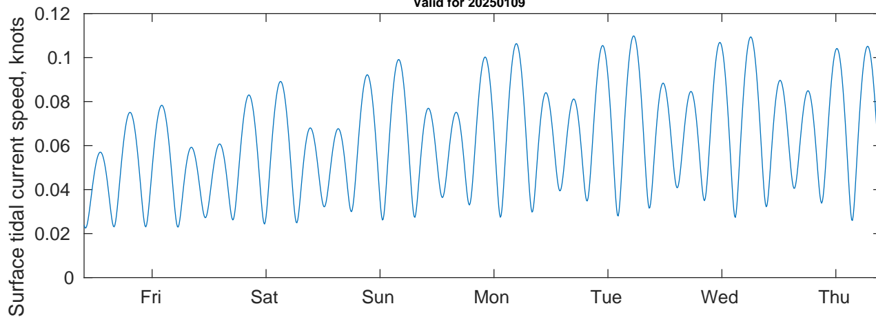
Tidal Currents and Heights for Nautilus at 20250109
