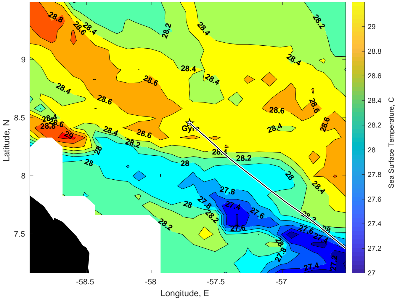
SST for Gyre at 09-Jan-2025 00:00:00
