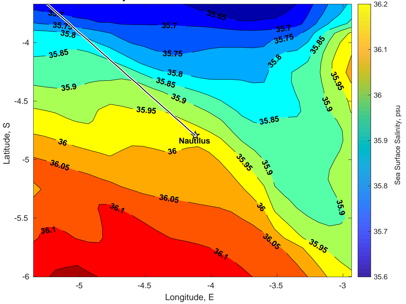
Surface Salinity for Nautilus at 09-Jan-2025 00:00:00
