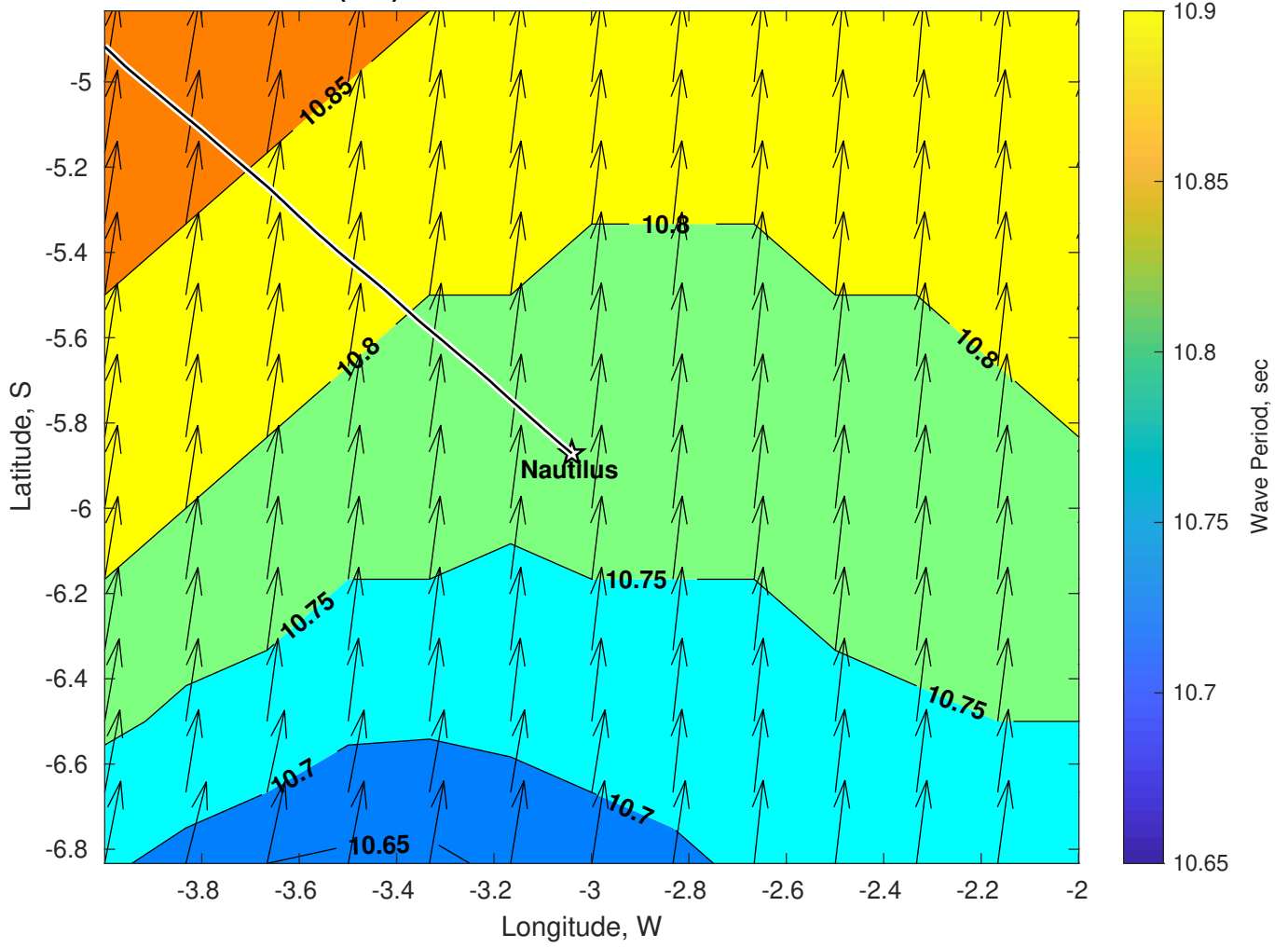
Wave Period (sec) for Nautilus at 10-Jan-2025 09:00:00
