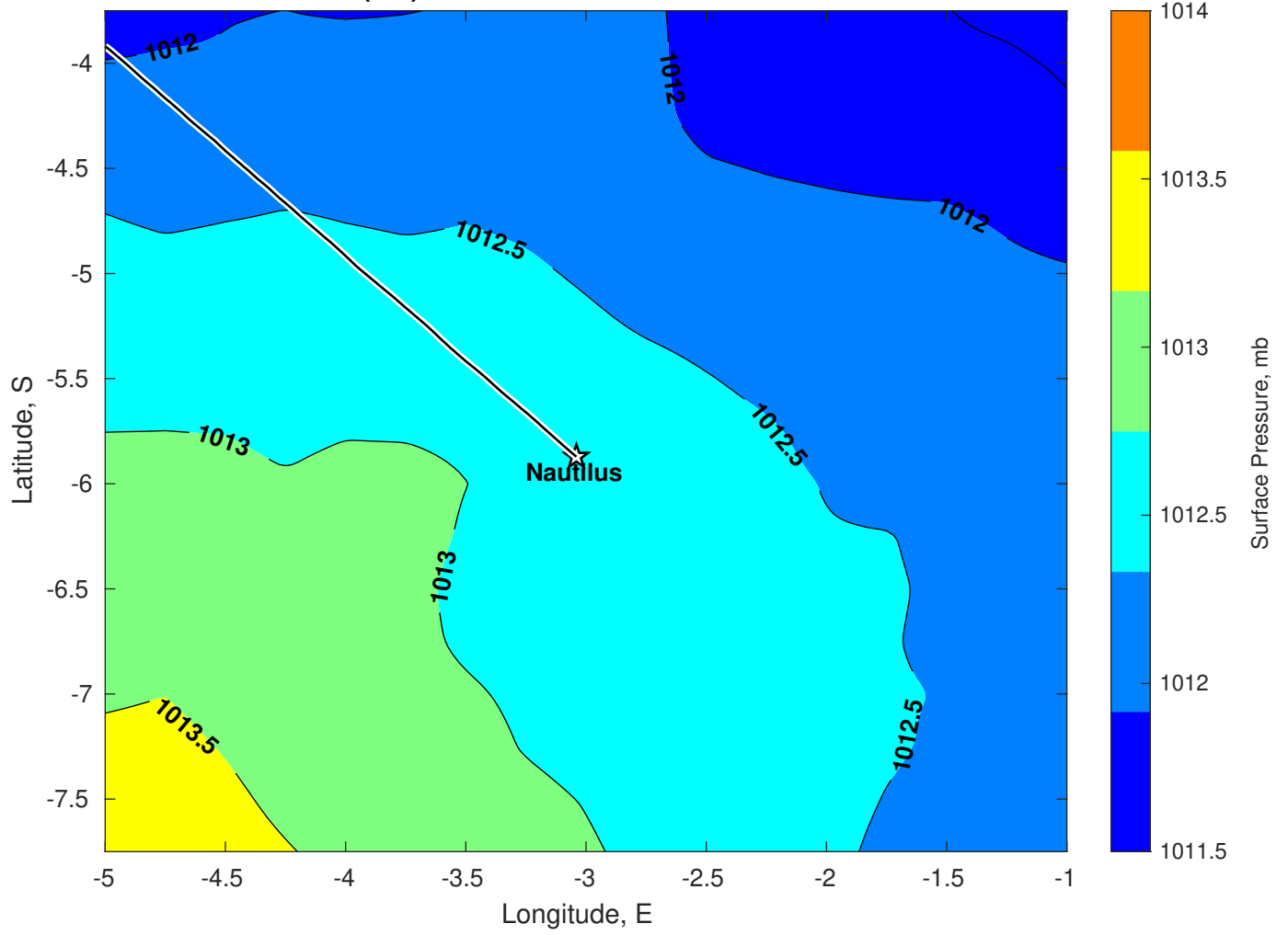
Surface Pressure (mb) for Nautilus at 11-Jan-2025 00:00:00
