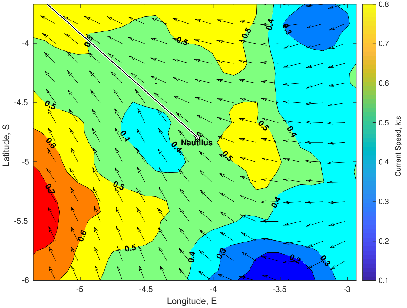
Surface Currents for Nautilus at 09-Jan-2025 00:00:00
