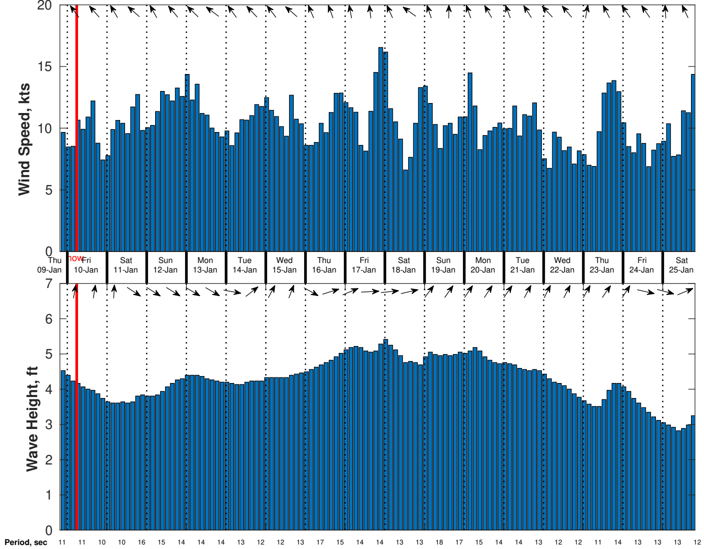
Wind & Wave Forecast for Nautilus from 09-Jan-2025 20:00:00 to 25-Jan-2025 20:00:00
