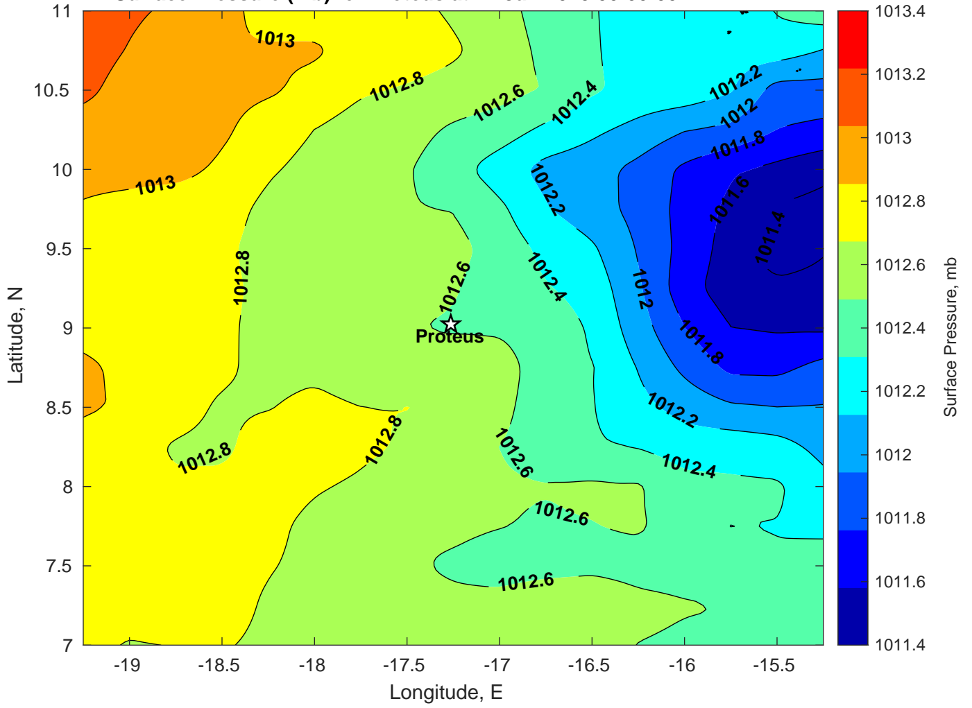
Surface Pressure (mb) for Proteus at 12-Jan-2025 00:00:00
