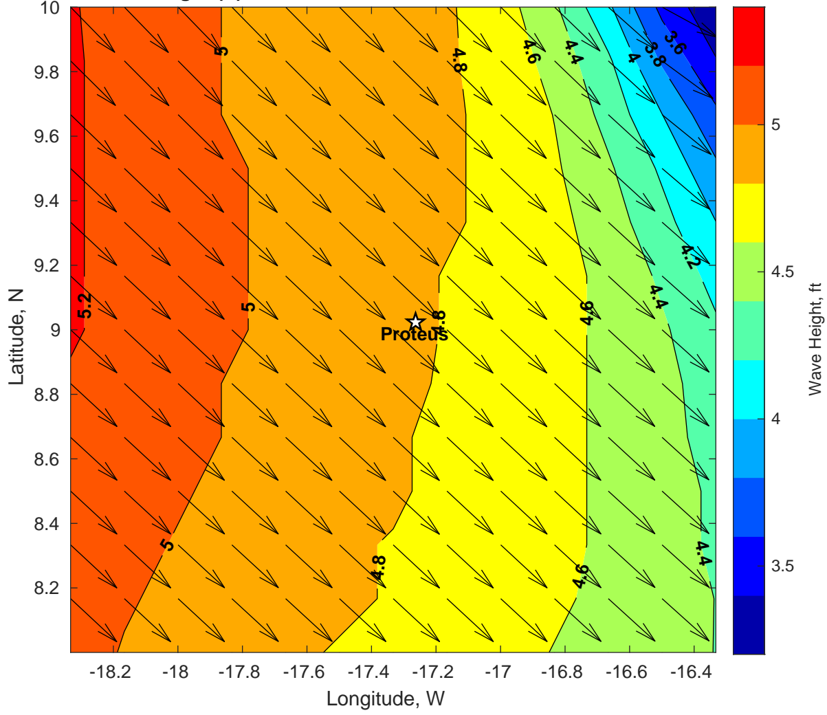
Wave Height (ft) for Proteus at 10-Jan-2025 09:00:00
