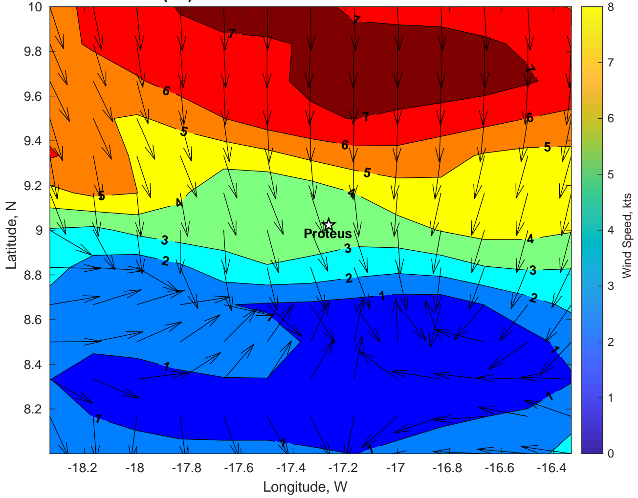
Winds (kts) for Proteus at 10-Jan-2025 09:00:00
