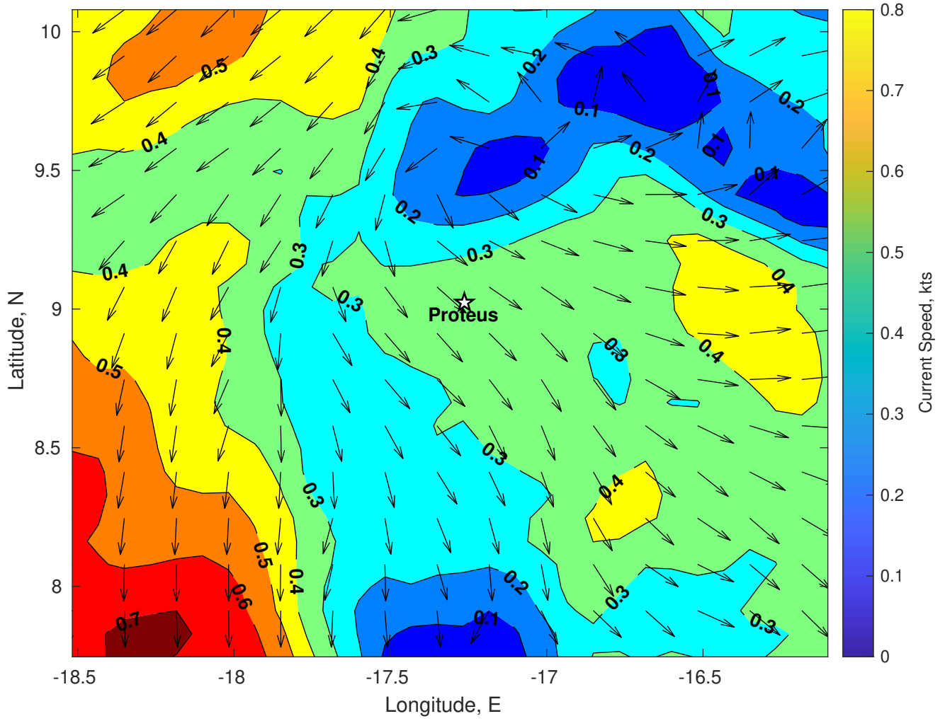
Surface Currents for Proteus at 09-Jan-2025 00:00:00
