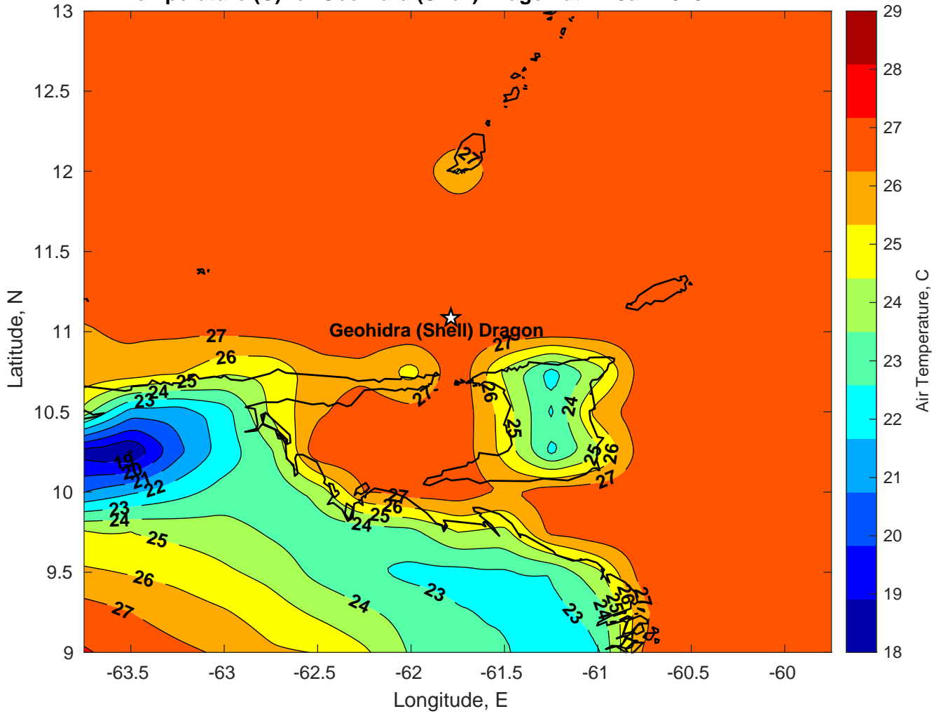
Air Temperature (C) for Geohidra (Shell) Dragon at 11-Jan-2025
