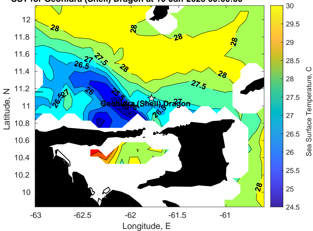
SST for Geohidra (Shell) Dragon at 10-Jan-2025 00:00:00
