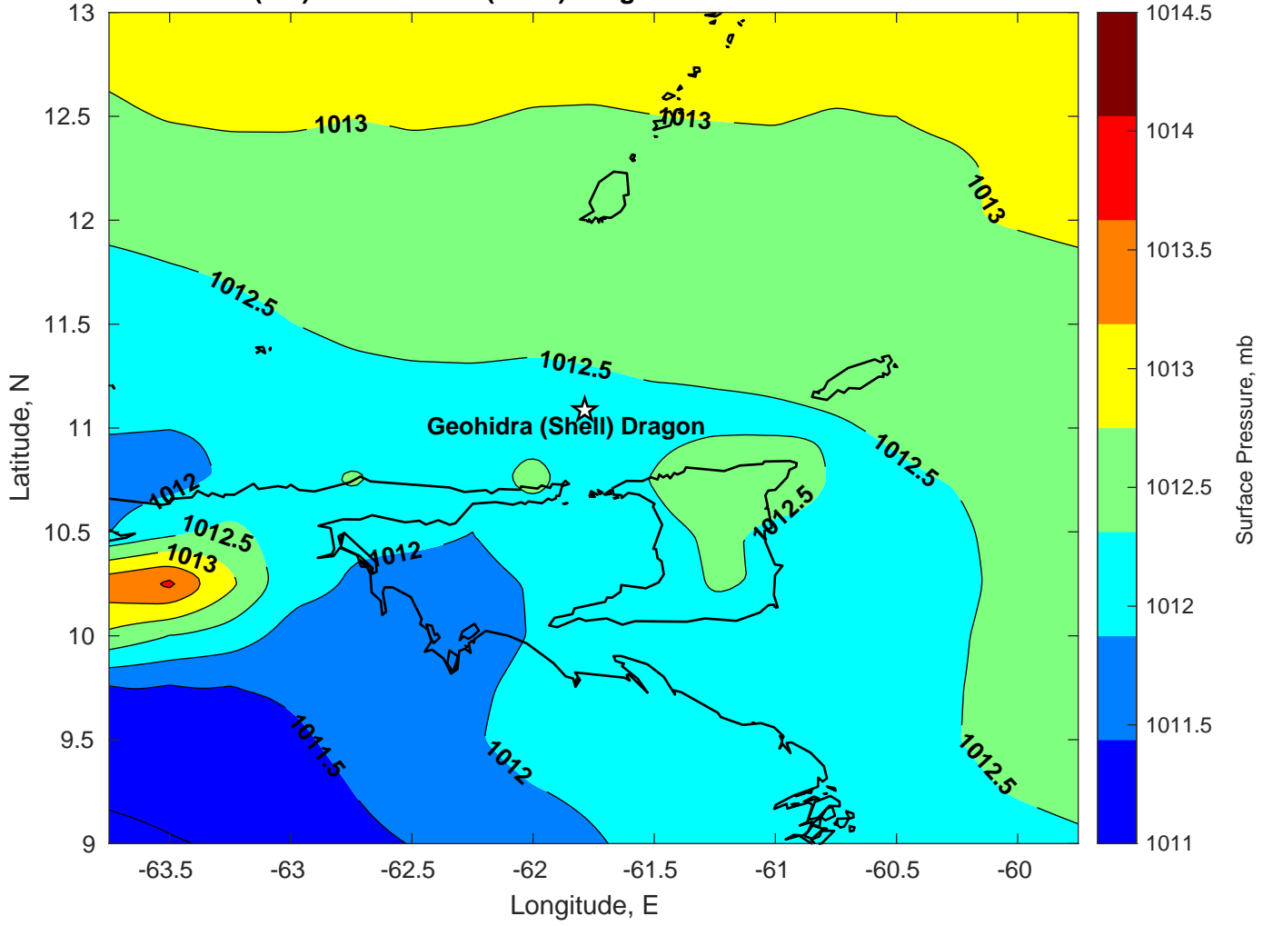
Surface Pressure (mb) for Geohidra (Shell) Dragon at 11-Jan-2025 00:00:00
