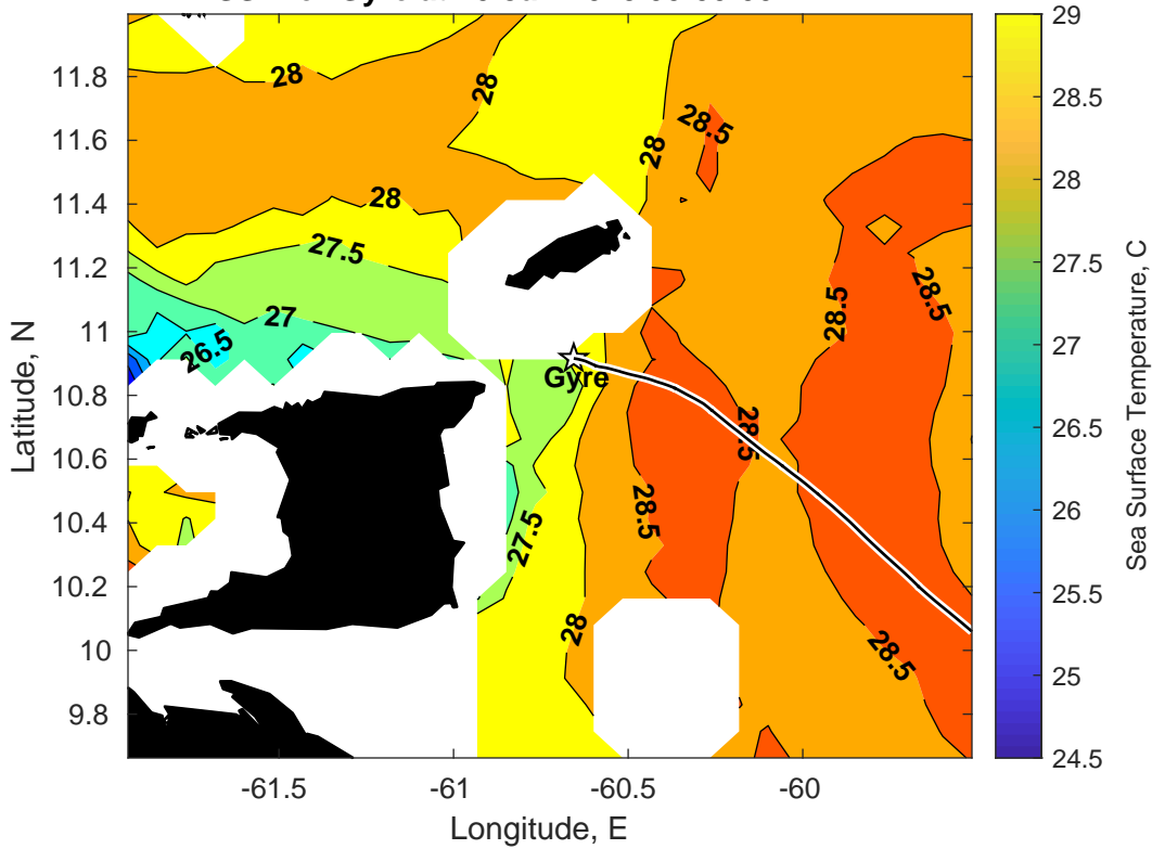
SST for Gyre at 10-Jan-2025 00:00:00
