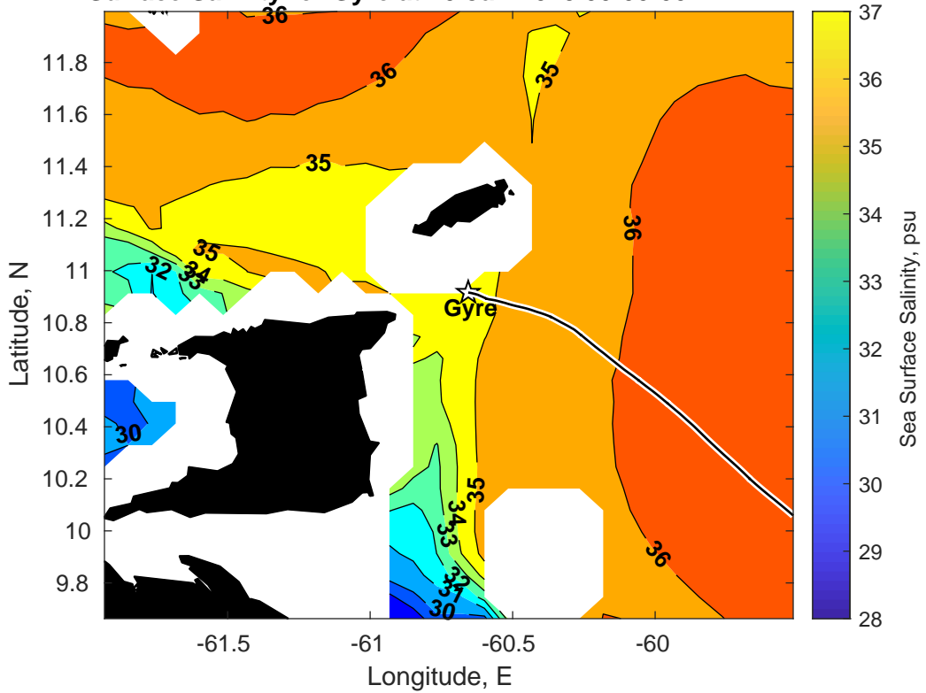
Surface Salinity for Gyre at 10-Jan-2025 00:00:00
