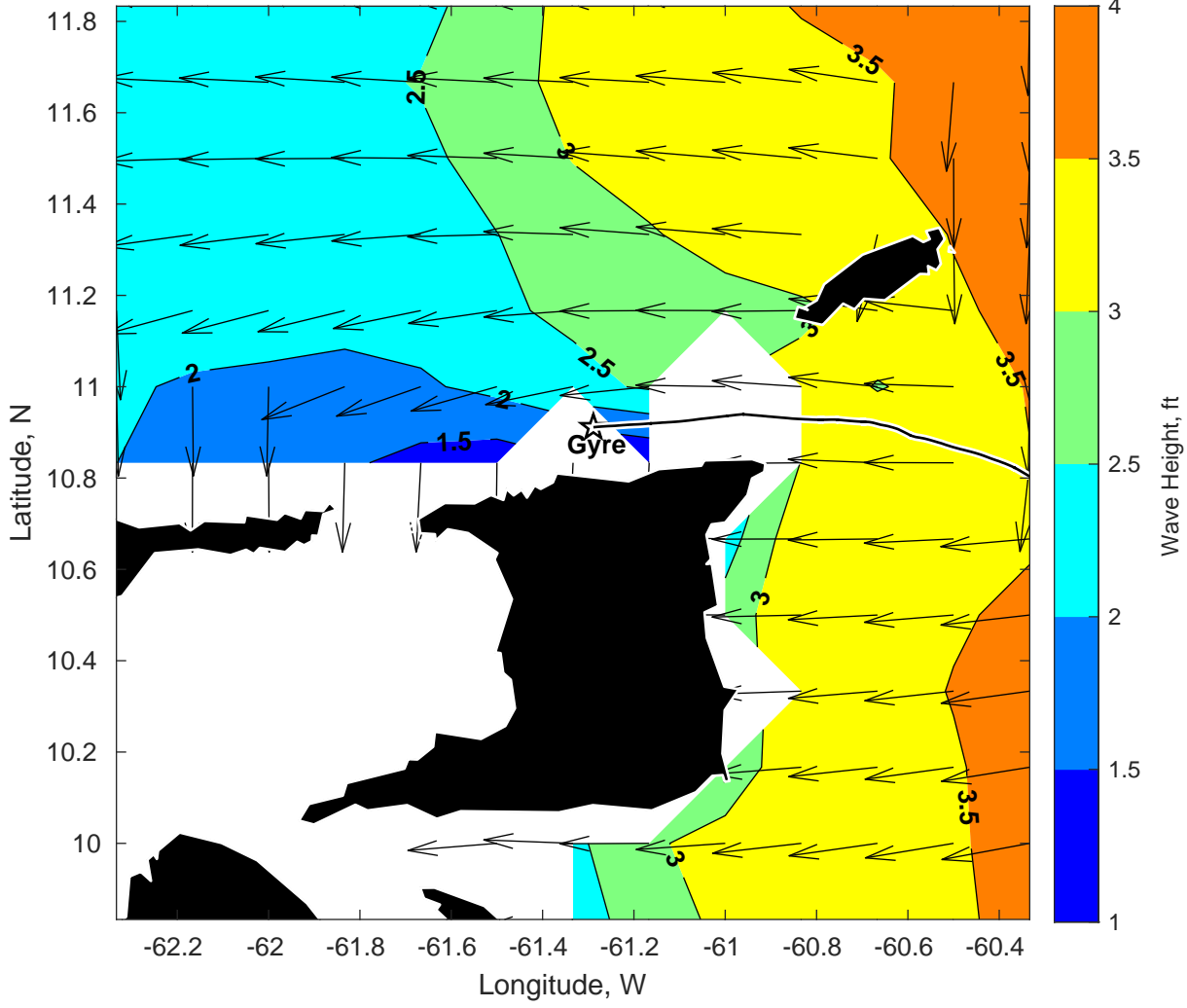
Wave Height (ft) for Gyre at 11-Jan-2025 09:00:00
