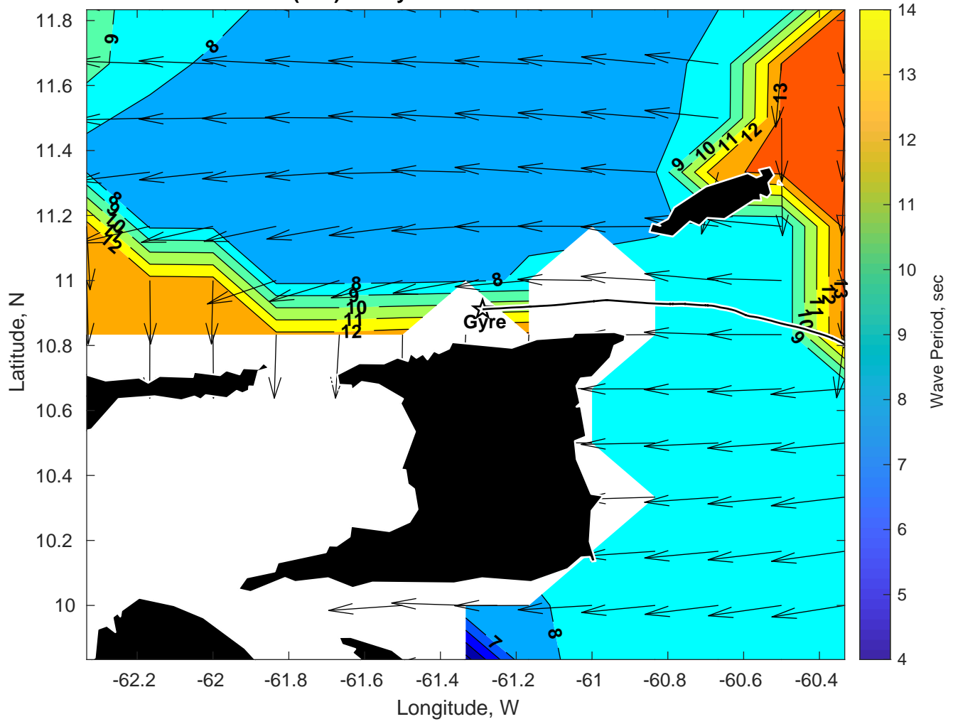
Wave Period (sec) for Gyre at 11-Jan-2025 09:00:00
