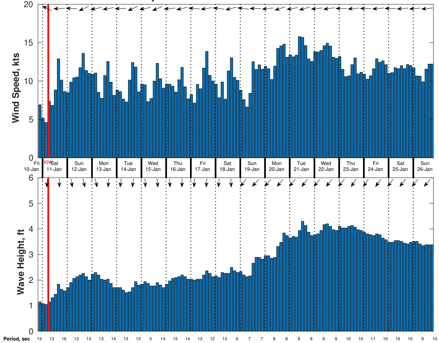
Wind & Wave Forecast for Gyre from 10-Jan-2025 20:00:00 to 26-Jan-2025 20:00:00
