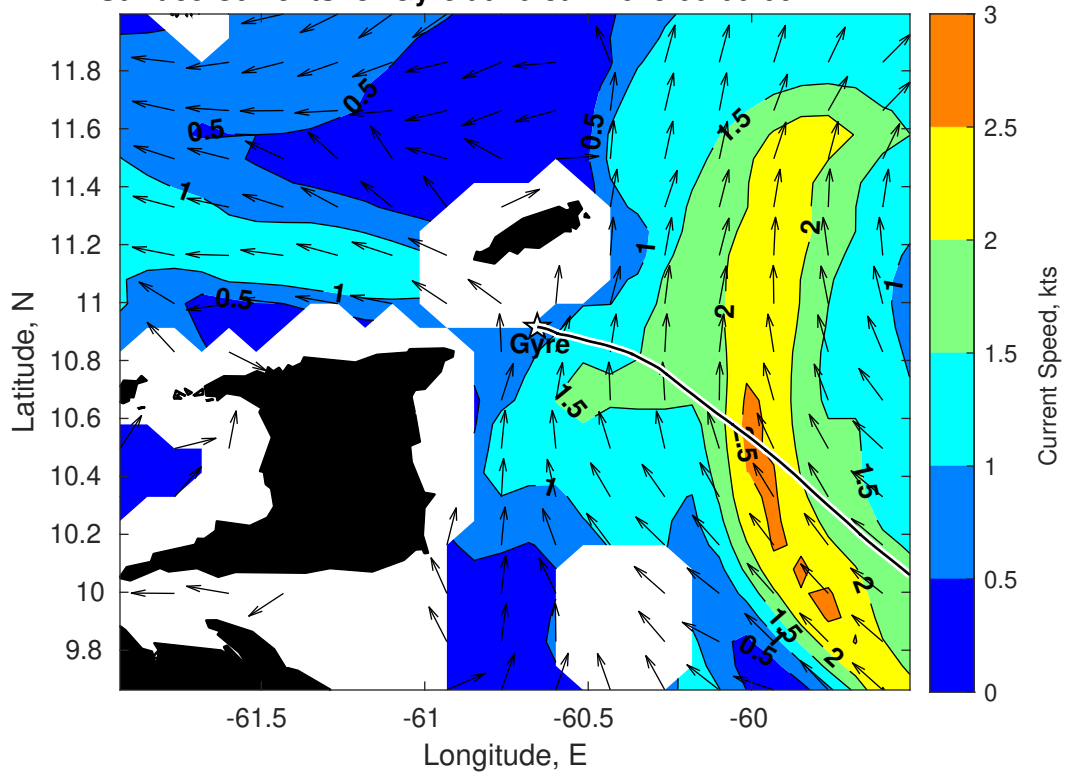
Surface Currents for Gyre at 10-Jan-2025 00:00:00
