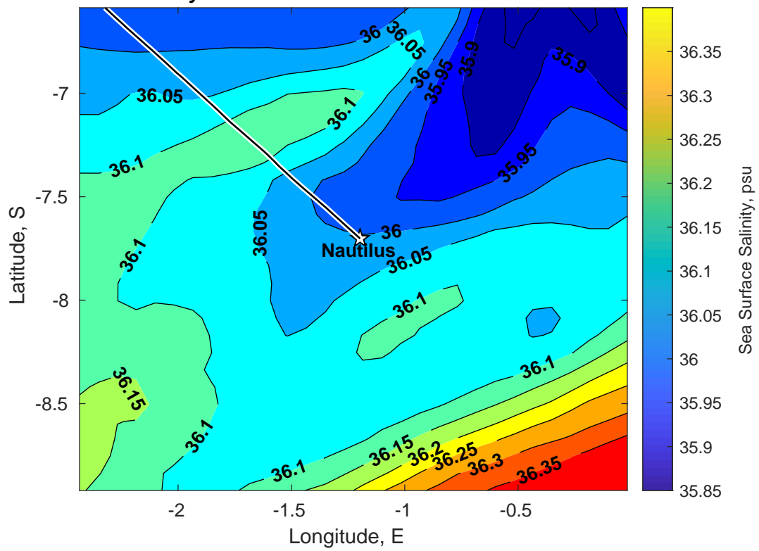
Surface Salinity for Nautilus at 10-Jan-2025 00:00:00
