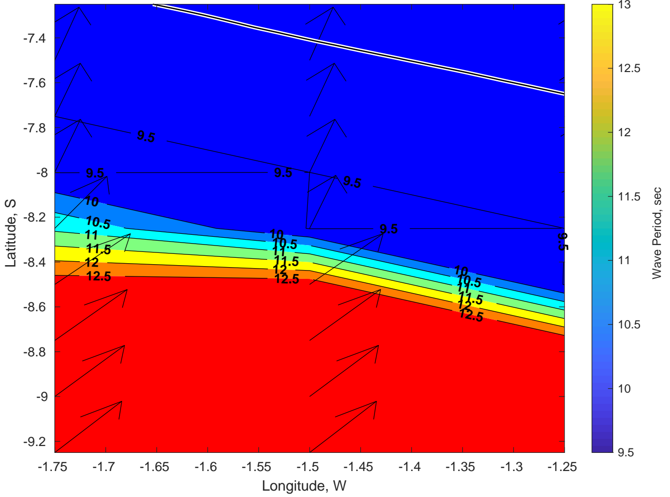
Wave Period (sec) for Nautilus at 11-Jan-2025 09:00:00
