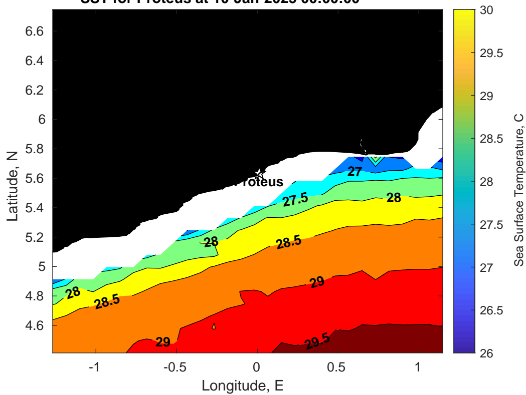
SST for Proteus at 10-Jan-2025 00:00:00
