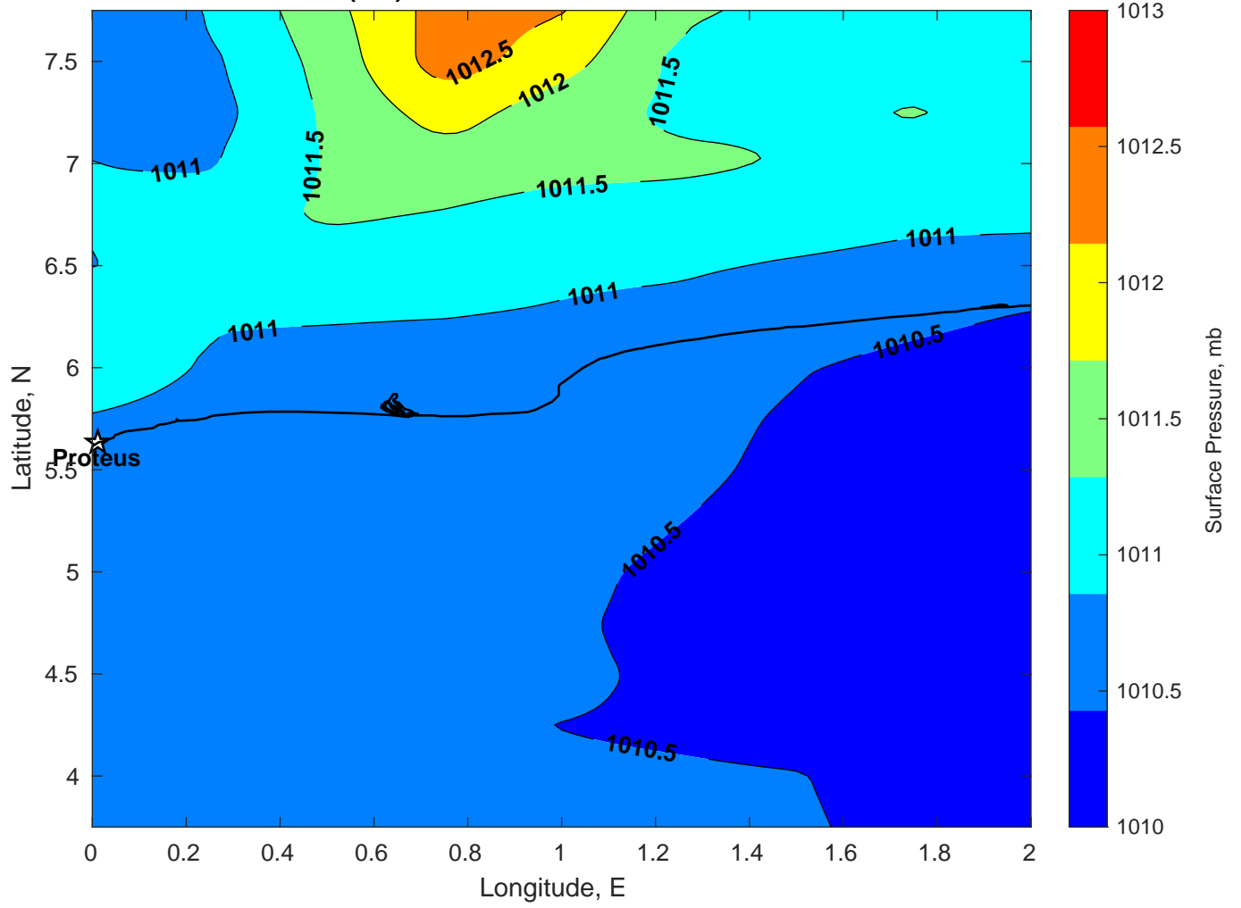
Surface Pressure (mb) for Proteus at 11-Jan-2025 00:00:00
