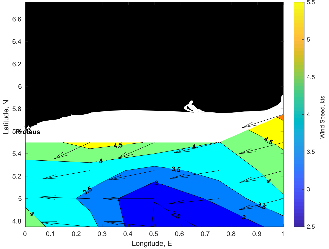
Winds (kts) for Proteus at 11-Jan-2025 09:00:00
