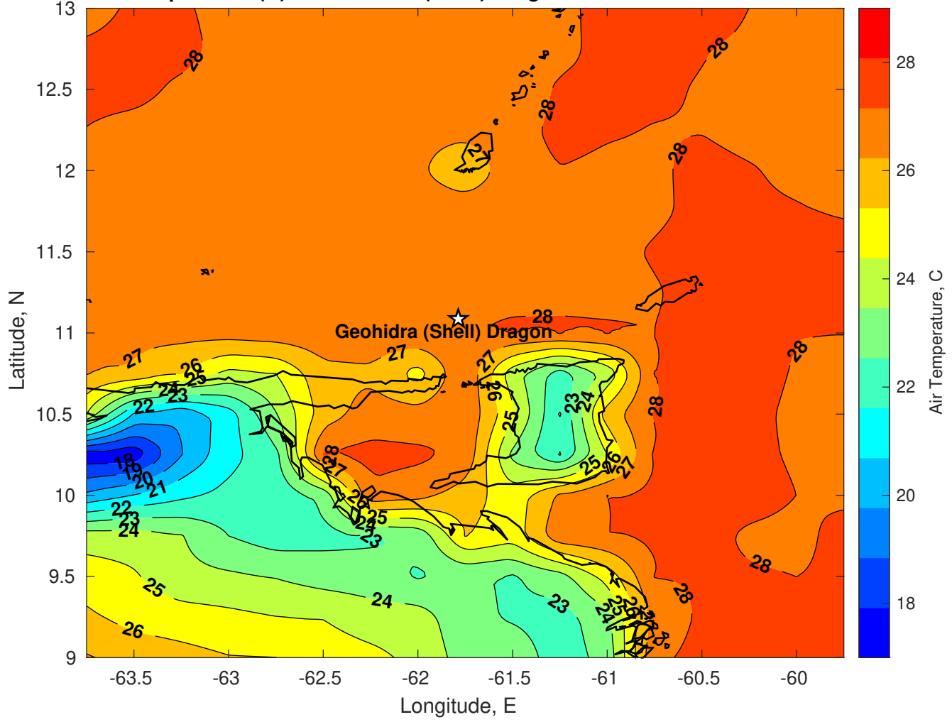
Air Temperature (C) for Geohidra (Shell) Dragon at 12-Jan-2025
