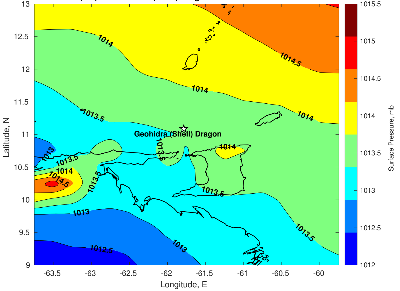
Surface Pressure (mb) for Geohidra (Shell) Dragon at 12-Jan-2025 00:00:00
