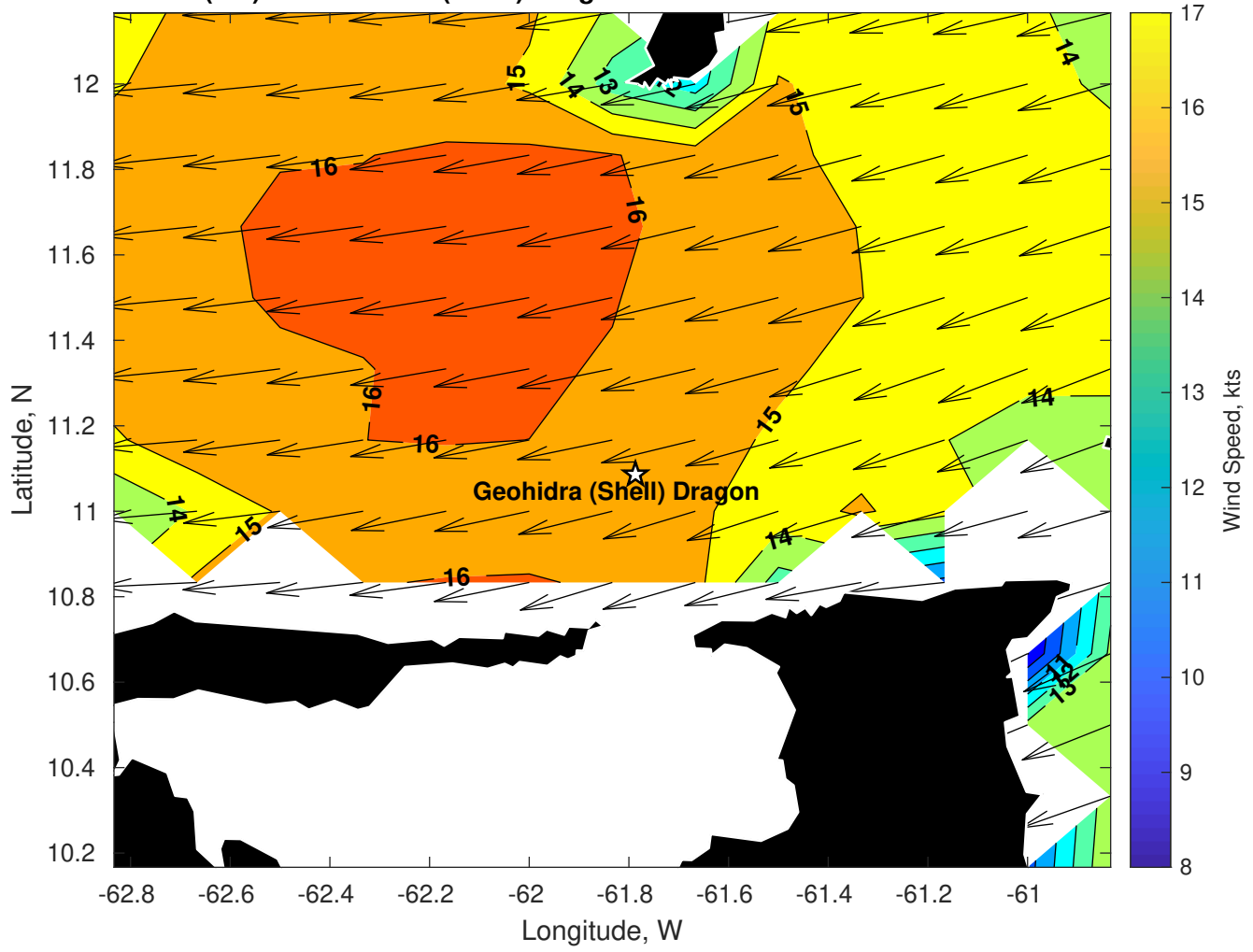
Winds (kts) for Geohidra (Shell) Dragon at 12-Jan-2025 09:00:00
