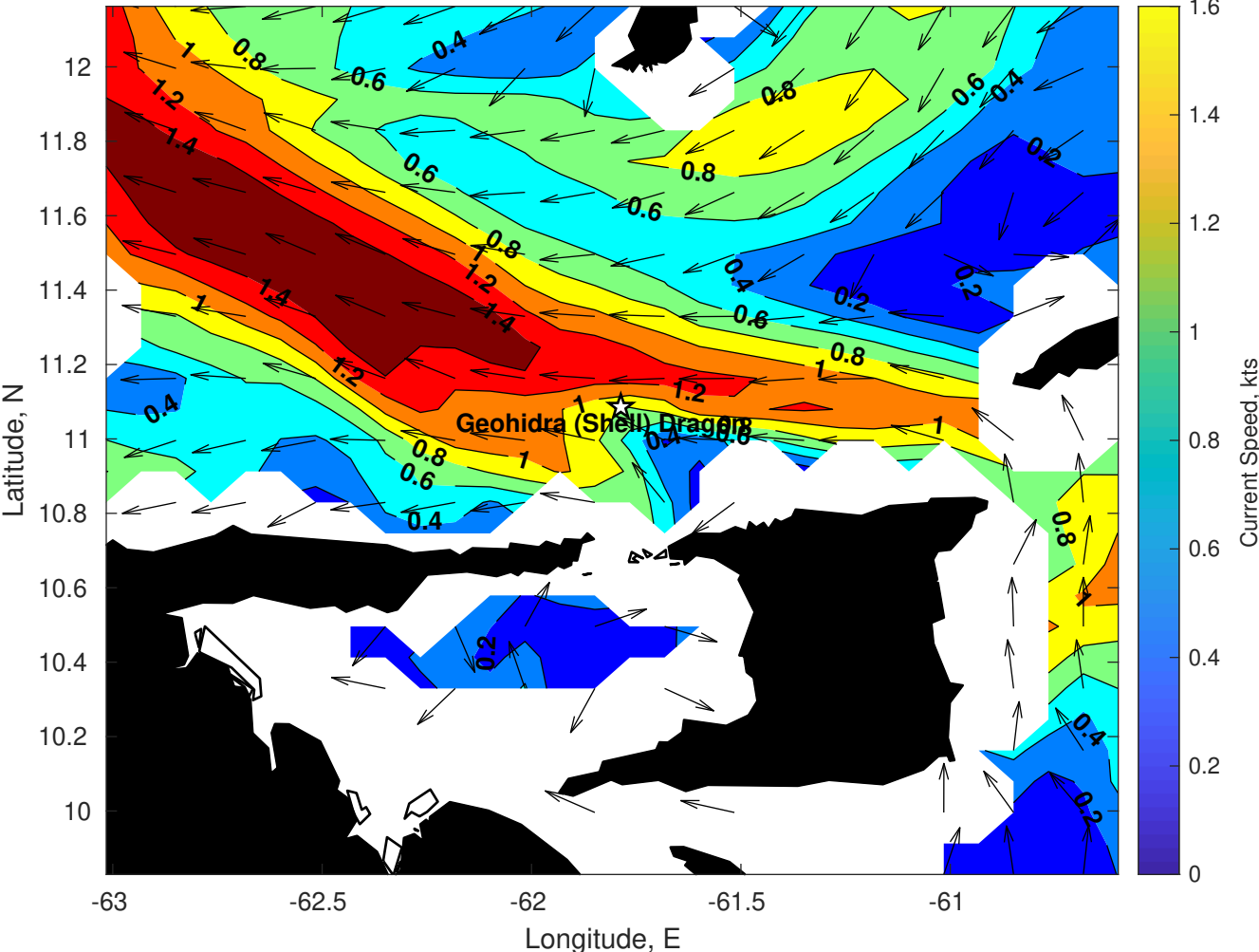
Surface Currents for Geohidra (Shell) Dragon at 11-Jan-2025 00:00:00
