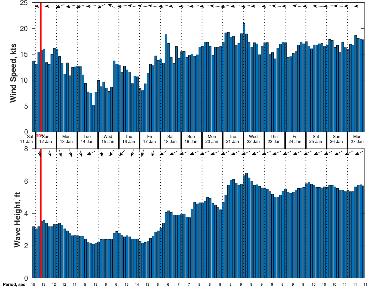
Wind & Wave Forecast for Geohidra (Shell) Dragon from 11-Jan-2025 20:00:00 to 27-Jan-2025 20:00:00
