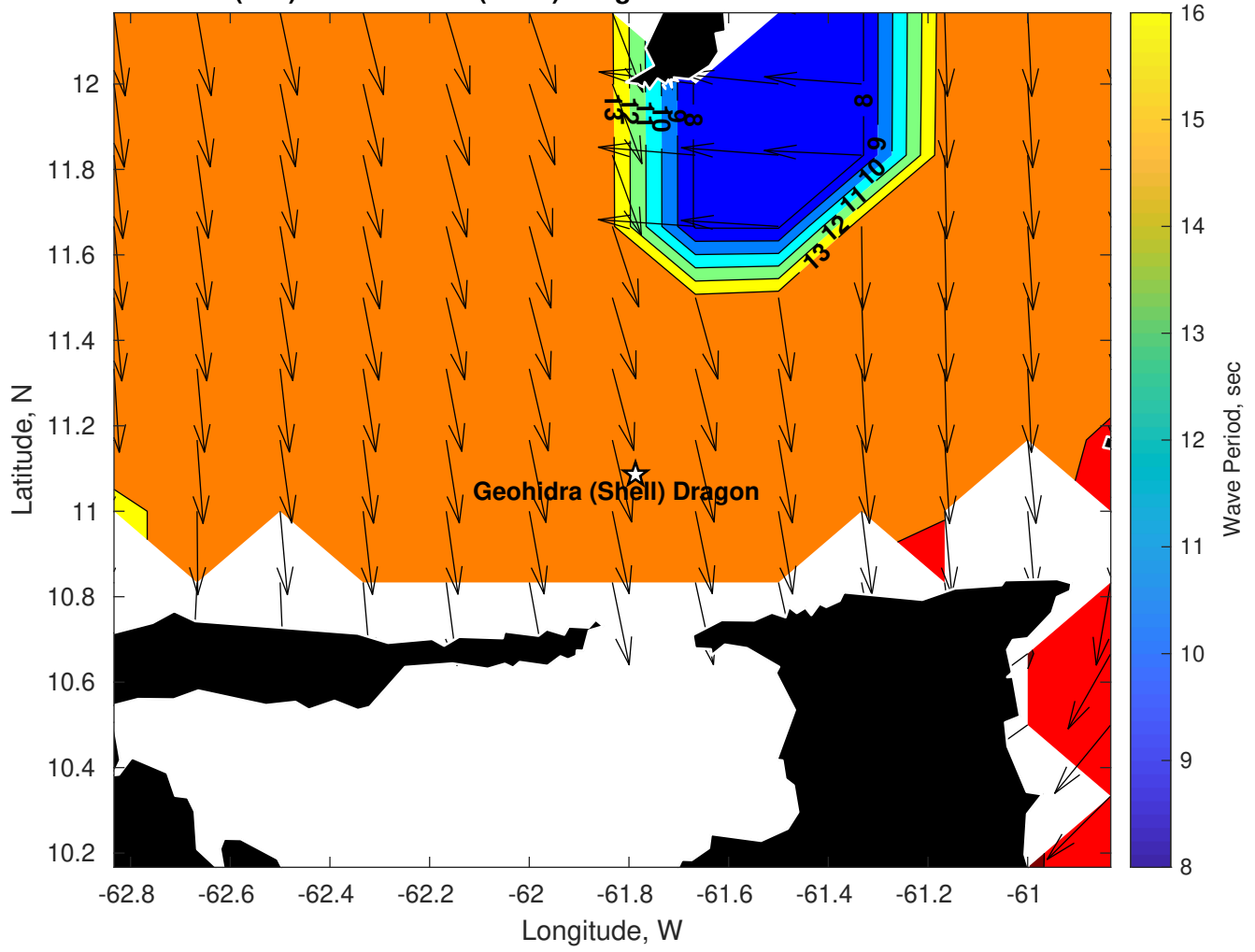
Wave Period (sec) for Geohidra (Shell) Dragon at 12-Jan-2025 09:00:00
