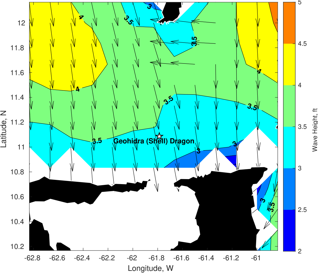
Wave Height (ft) for Geohidra (Shell) Dragon at 12-Jan-2025 09:00:00
