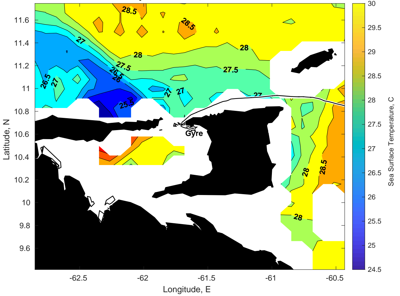
SST for Gyre at 11-Jan-2025 00:00:00
