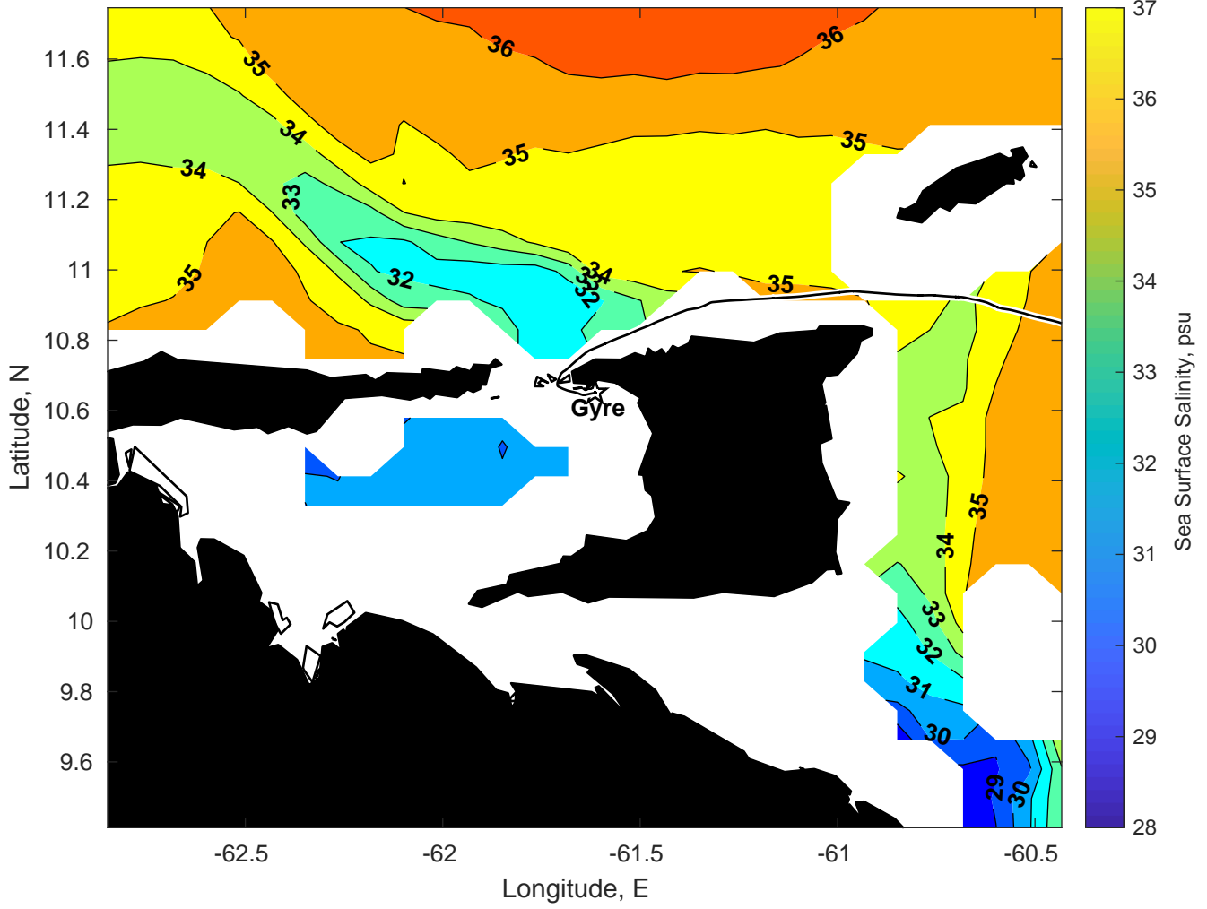
Surface Salinity for Gyre at 11-Jan-2025 00:00:00
