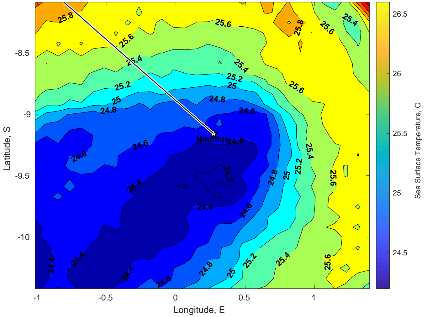
SST for Nautilus at 11-Jan-2025 00:00:00
