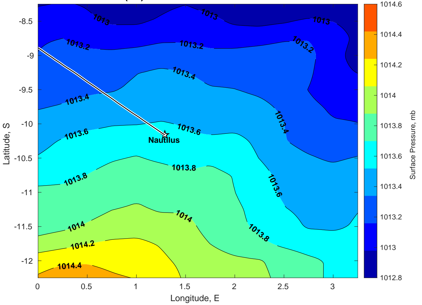
Surface Pressure (mb) for Nautilus at 12-Jan-2025 00:00:00
