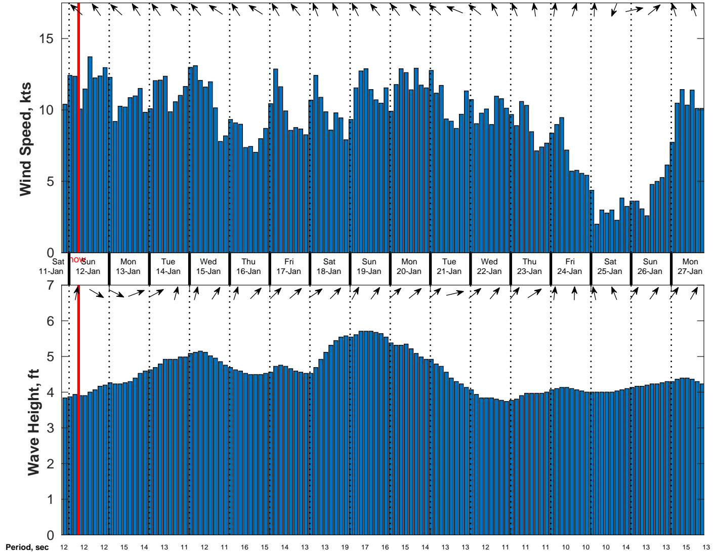
Wind & Wave Forecast for Nautilus from 11-Jan-2025 20:00:00 to 27-Jan-2025 20:00:00
