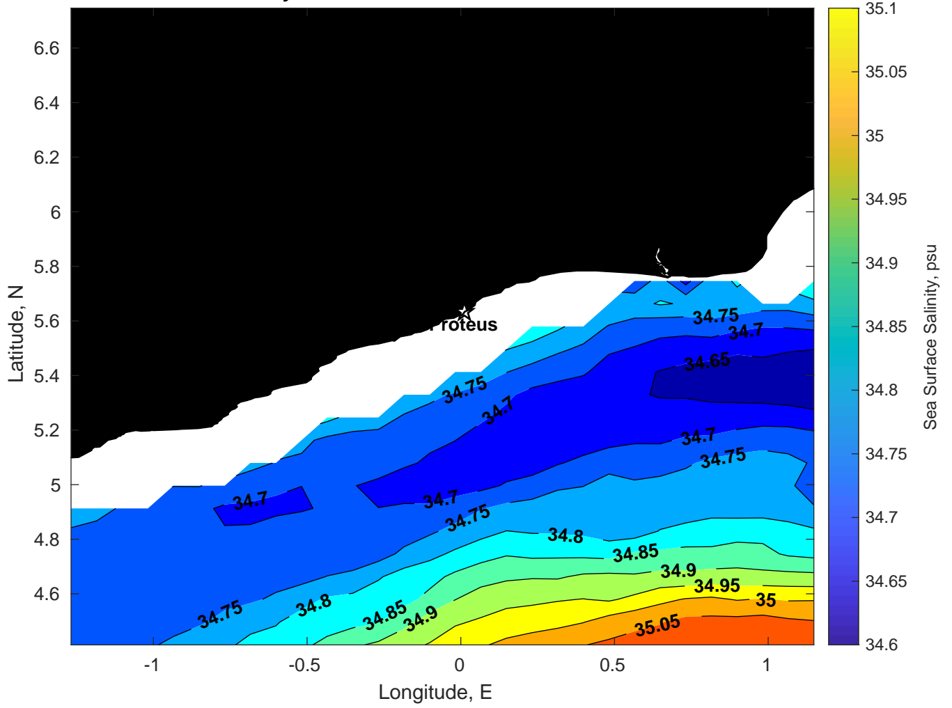
Surface Salinity for Proteus at 11-Jan-2025 00:00:00
