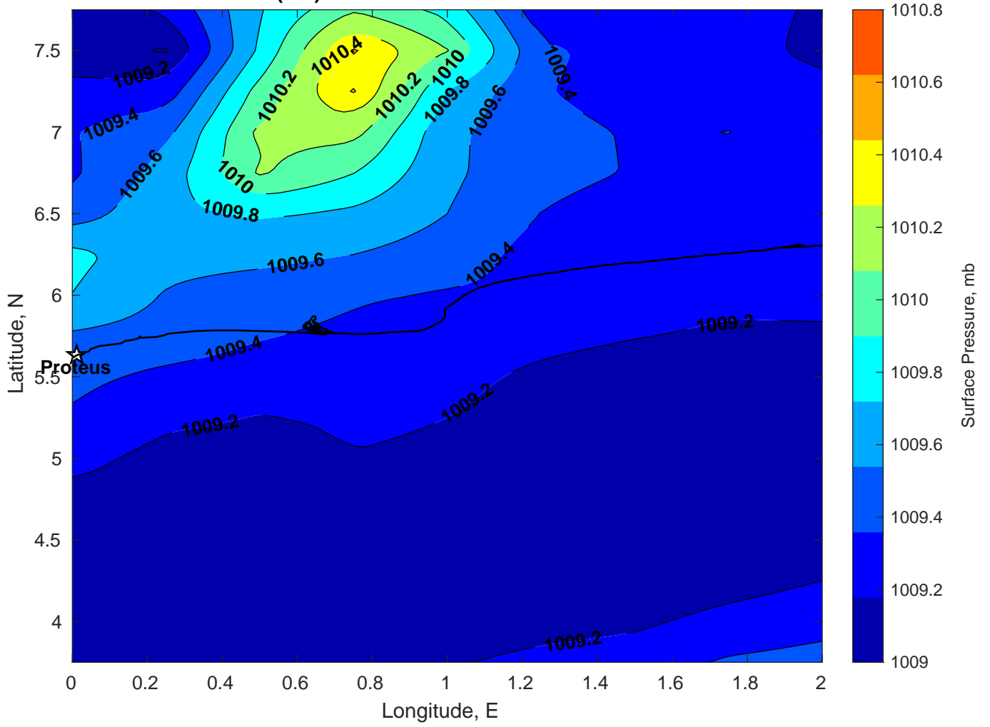
Surface Pressure (mb) for Proteus at 14-Jan-2025 00:00:00
