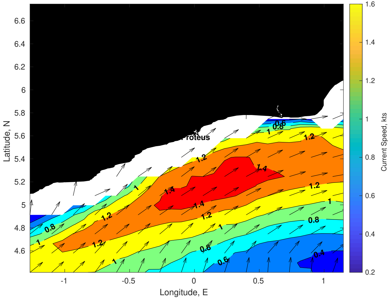
Surface Currents for Proteus at 11-Jan-2025 00:00:00
