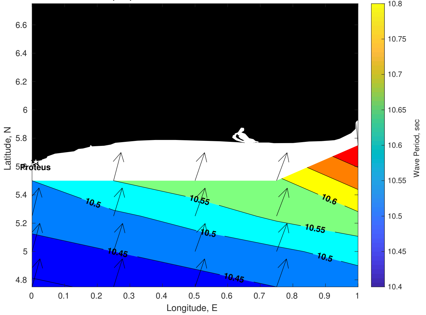
Wave Period (sec) for Proteus at 12-Jan-2025 09:00:00
