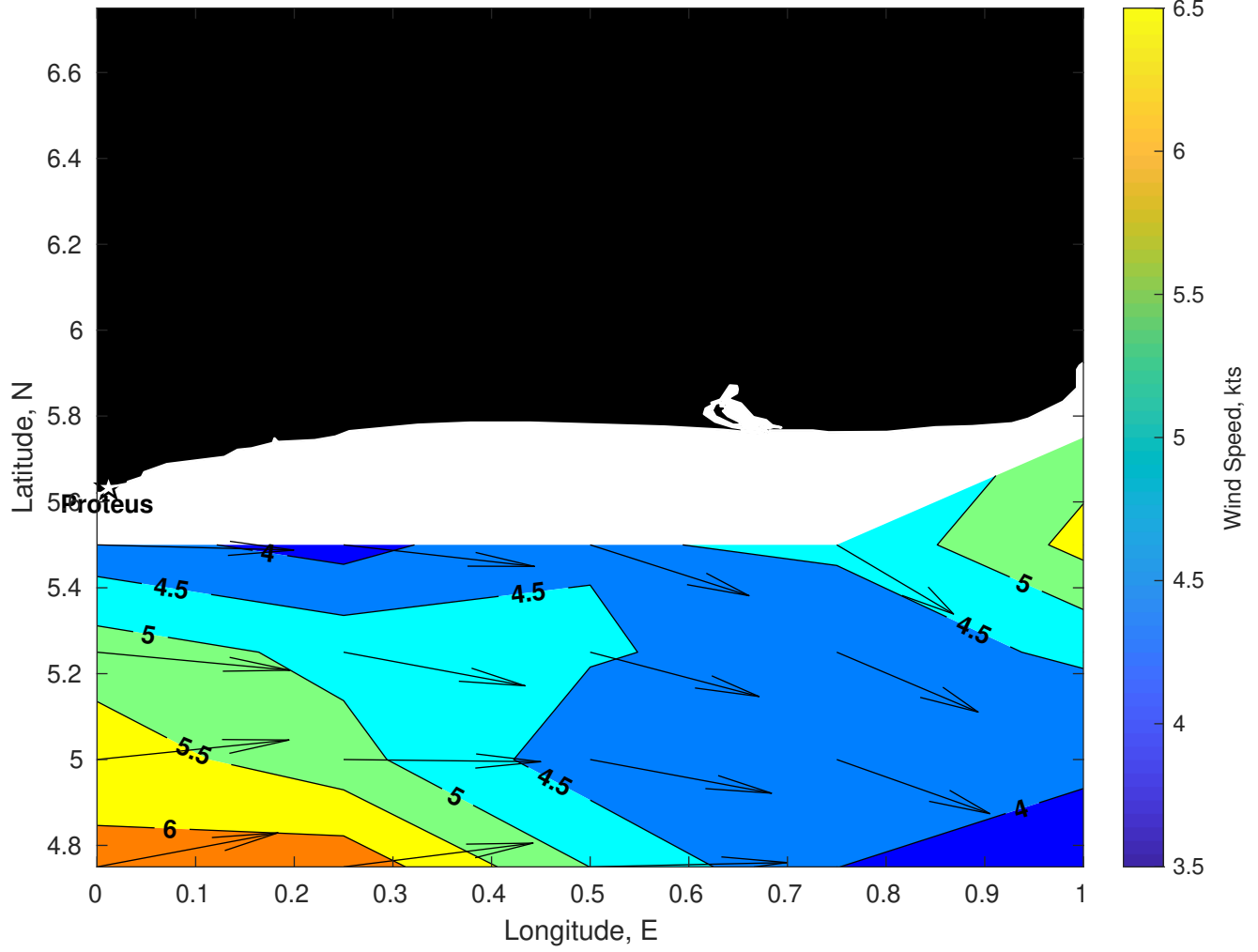
Winds (kts) for Proteus at 12-Jan-2025 09:00:00
