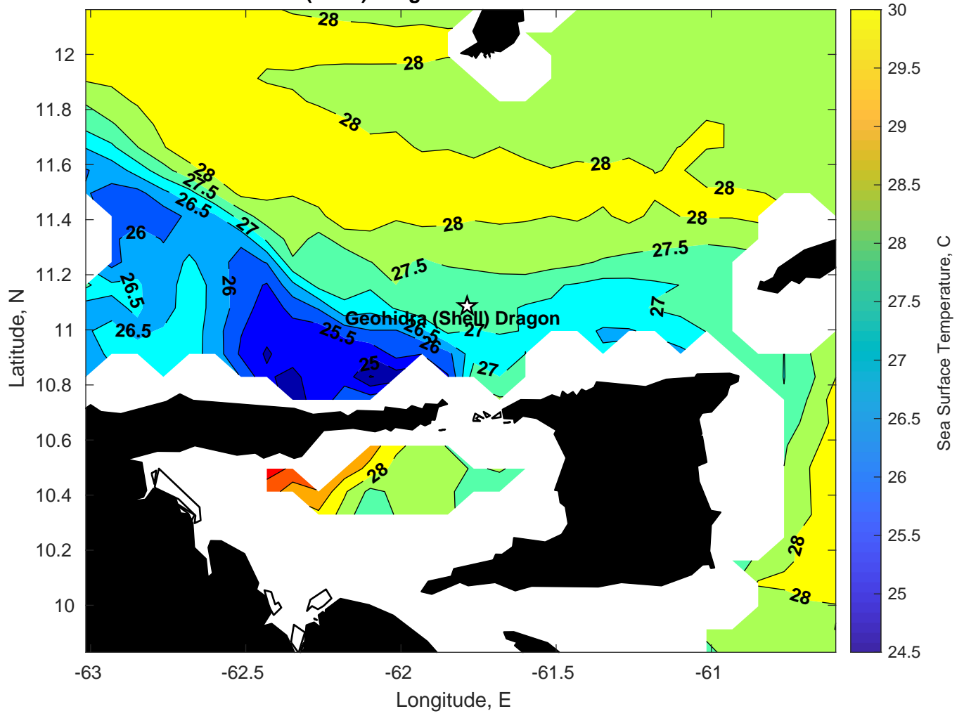
SST for Geohidra (Shell) Dragon at 12-Jan-2025 00:00:00
