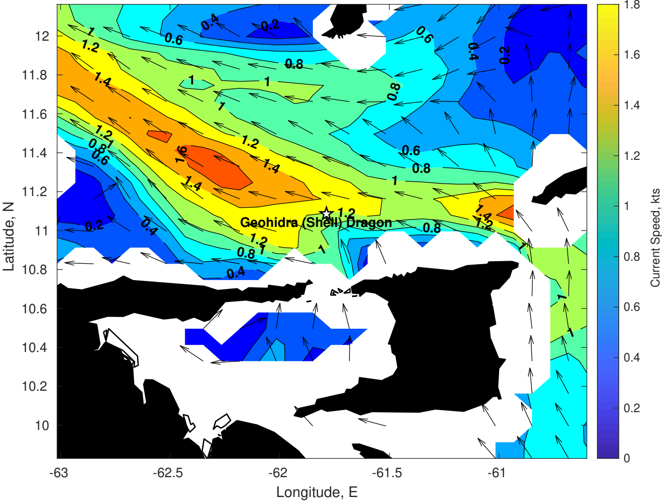
Surface Currents for Geohidra (Shell) Dragon at 12-Jan-2025 00:00:00
