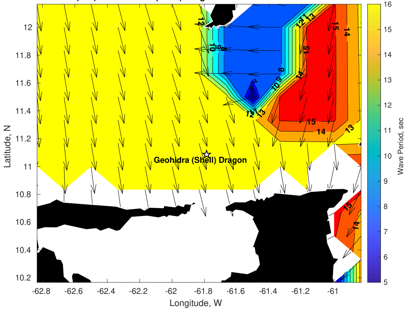
Wave Period (sec) for Geohidra (Shell) Dragon at 13-Jan-2025 09:00:00
