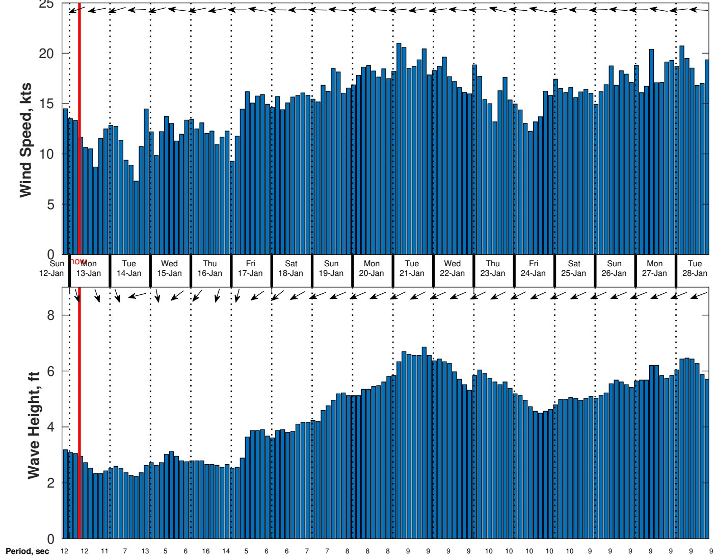
Wind & Wave Forecast for Geohidra (Shell) Dragon from 12-Jan-2025 20:00:00 to 28-Jan-2025 20:00:00
