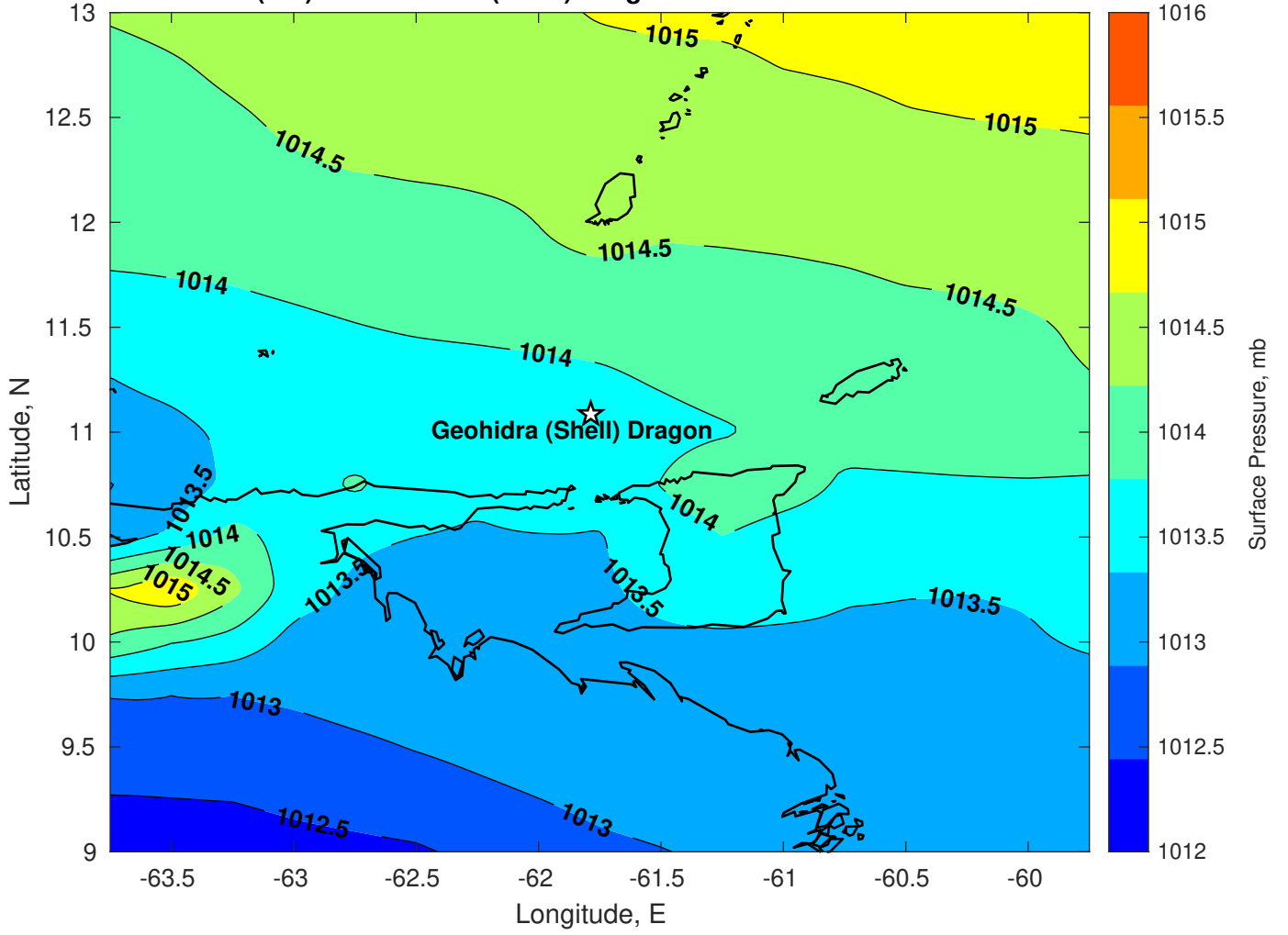
Surface Pressure (mb) for Geohidra (Shell) Dragon at 13-Jan-2025 00:00:00
