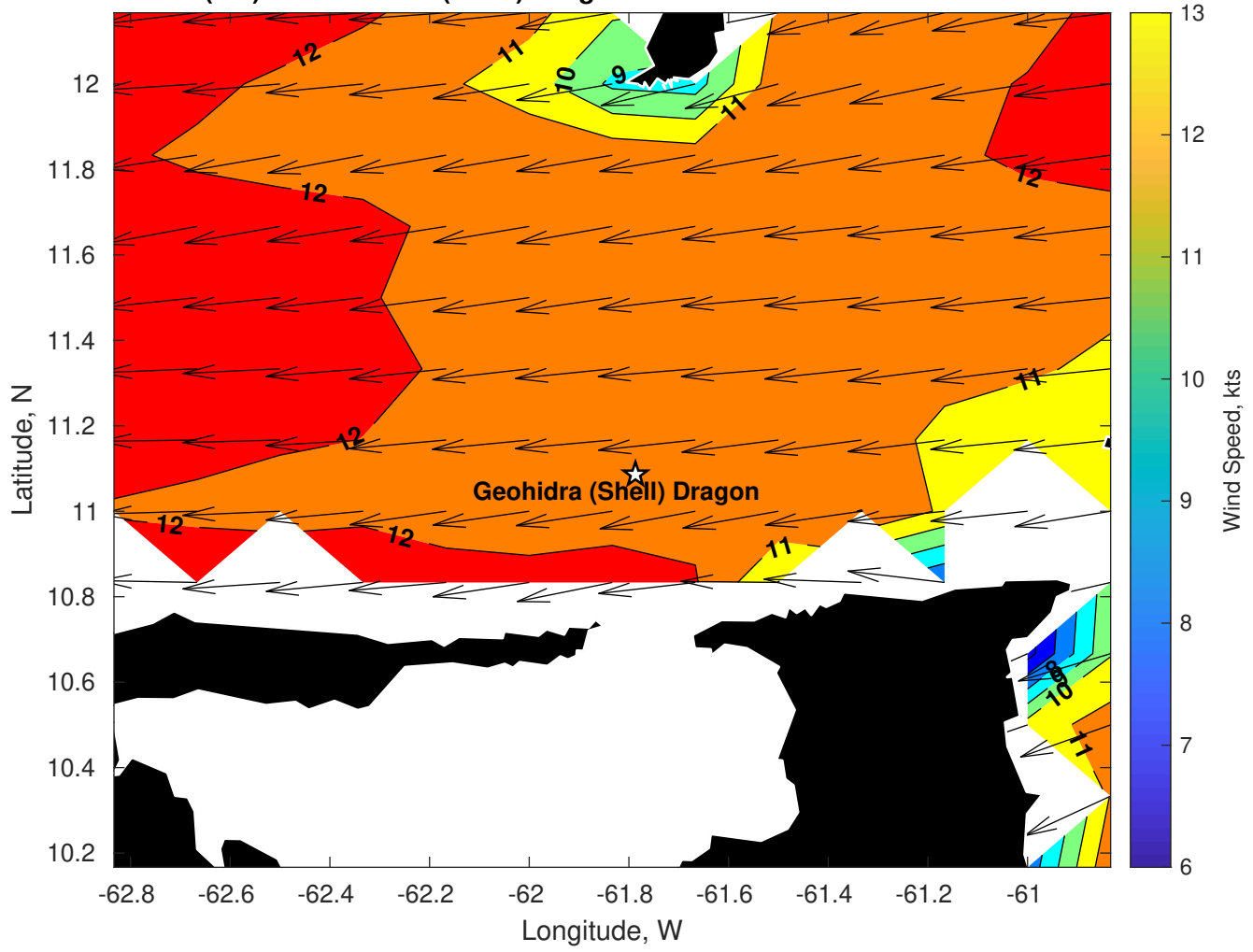
Winds (kts) for Geohidra (Shell) Dragon at 13-Jan-2025 09:00:00
