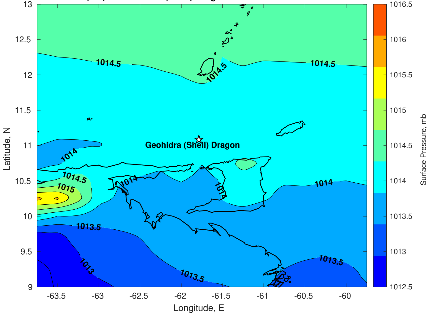
Surface Pressure (mb) for Geohidra (Shell) Dragon at 14-Jan-2025 00:00:00
