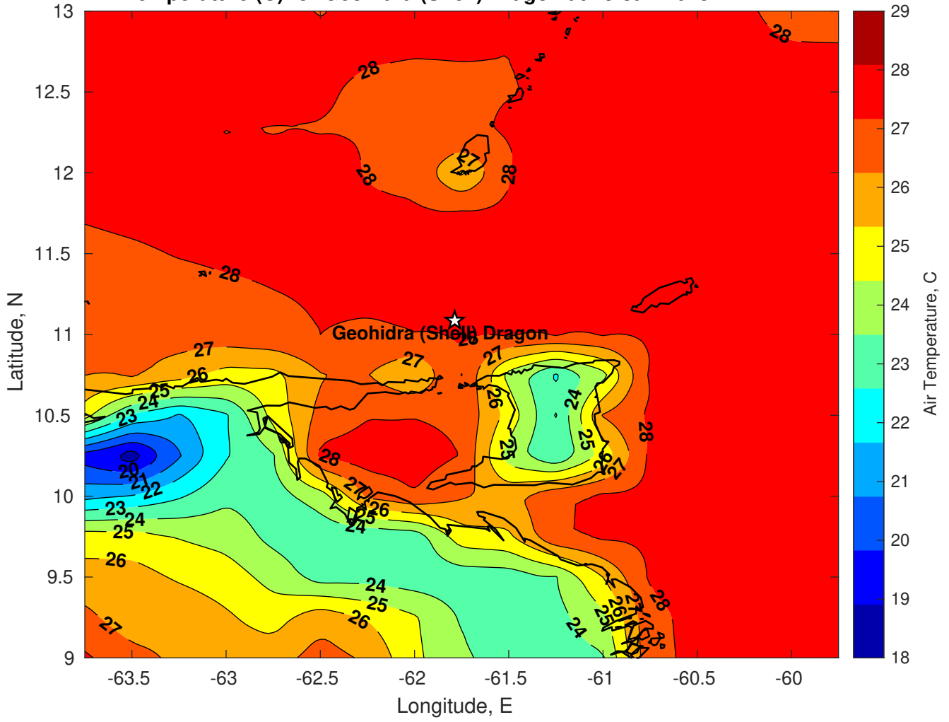
Air Temperature (C) for Geohidra (Shell) Dragon at 13-Jan-2025
