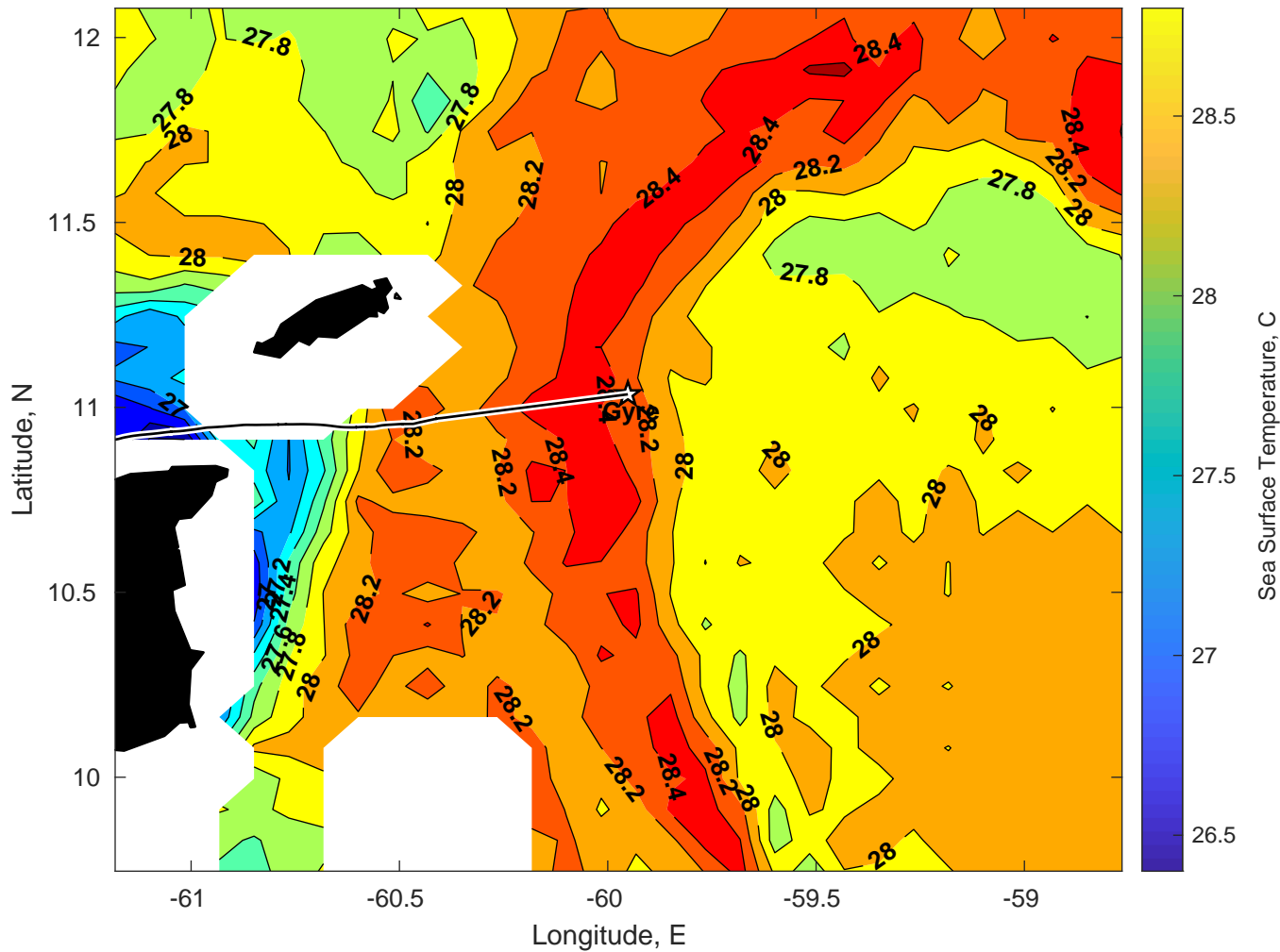
SST for Gyre at 12-Jan-2025 00:00:00
